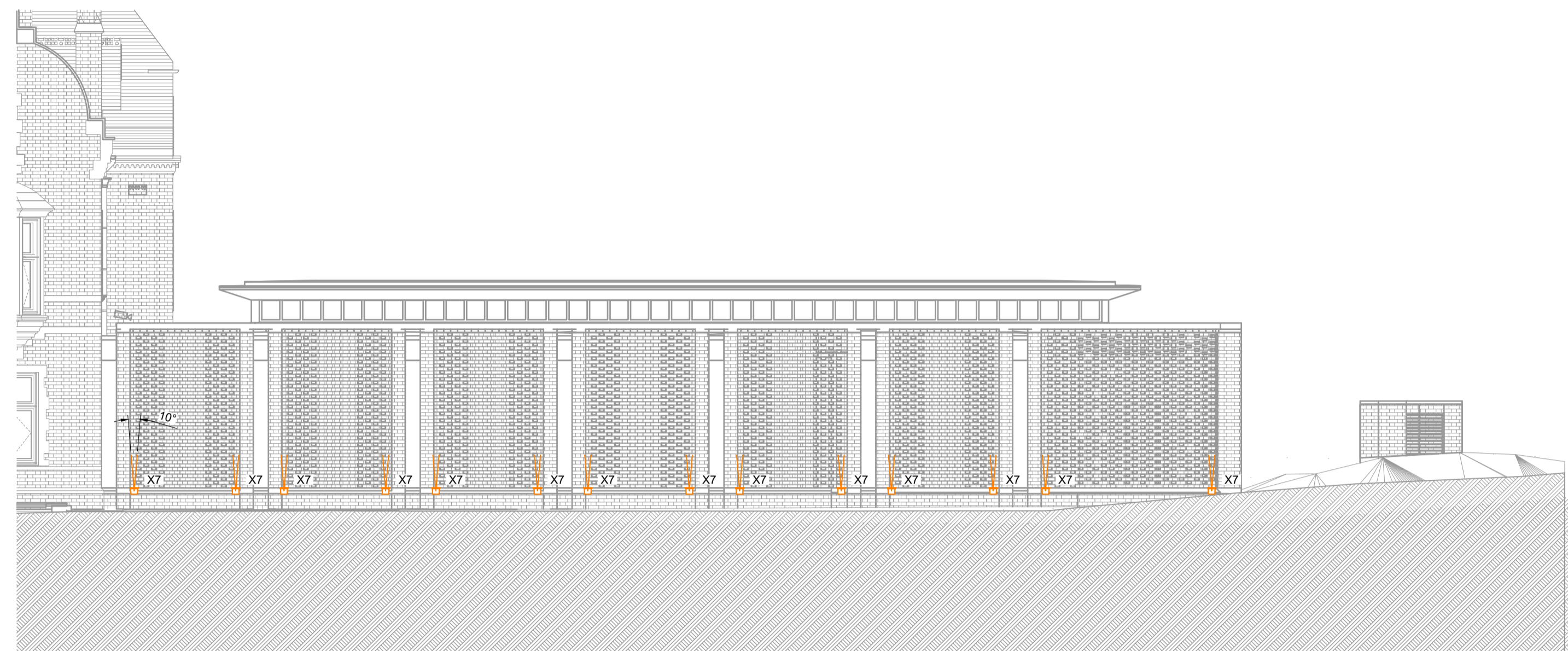
E East Elevation New Wing
