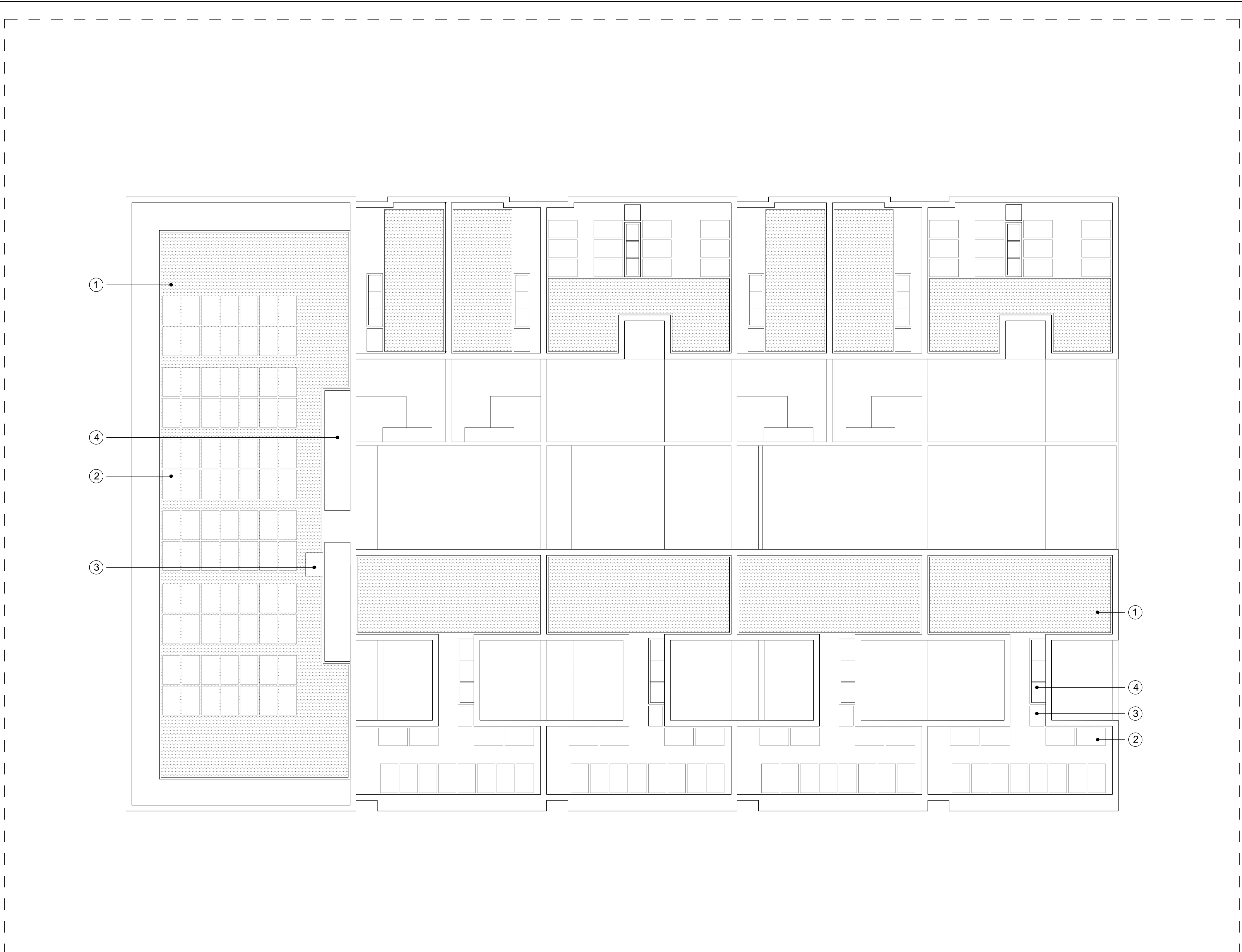
01 Proposed Block Plan - Roof Level
