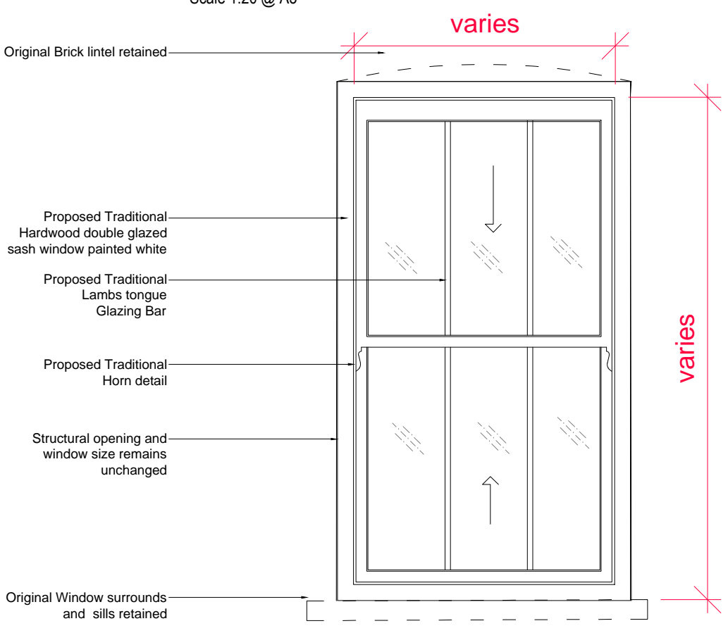
TYPE 04 - PROPOSED WINDOW - BACK ELEVATION Scale 1:20 @ A3
