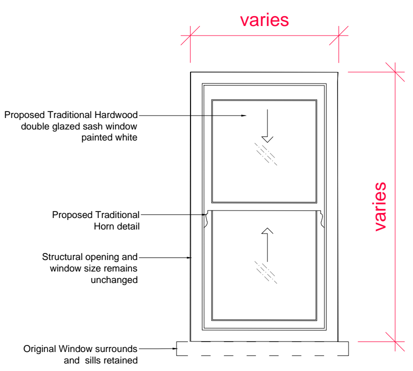
TYPE 05 - PROPOSED WINDOW - SIDE ELEVATION Scale 1:20 @ A3
