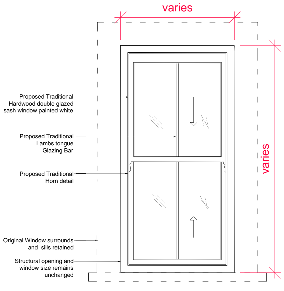
TYPE 02 - PROPOSED WINDOW - FRONT ELEVATION Scale 1:20 @ A3
