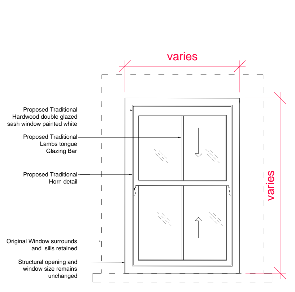
TYPE 03 - PROPOSED WINDOW - FRONT ELEVATION Scale 1:20 @ A3
