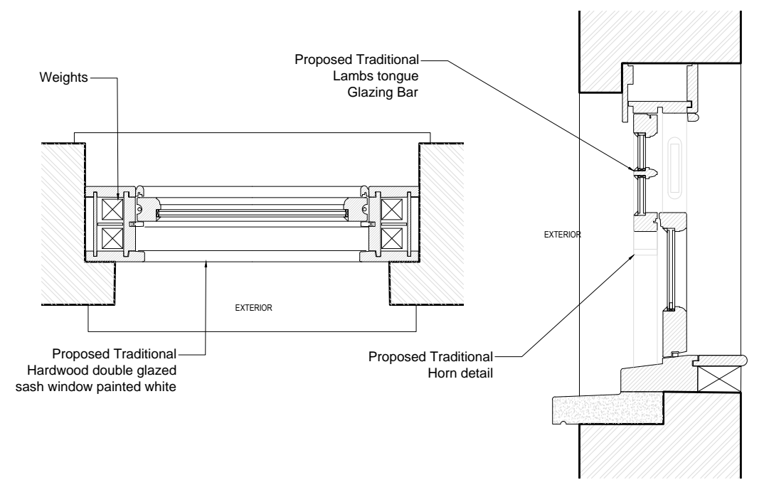
TYPICAL SASH DETAIL Scale 1:10 @ A3
