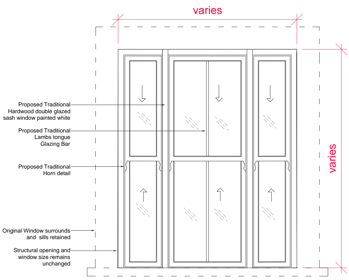
TYPE 01 - PROPOSED WINDOW - FRONT ELEVATION Scale 1:20 @ A3
