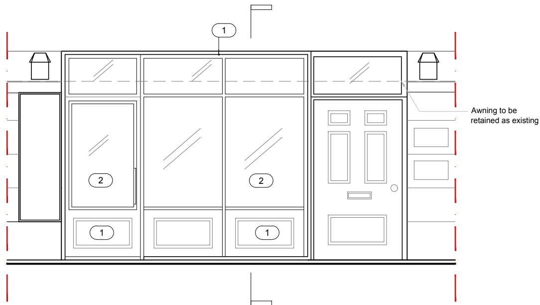
1 Proposed Elevation 1:50
