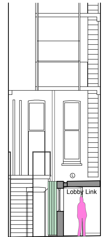
99.00 SECTION C - C
