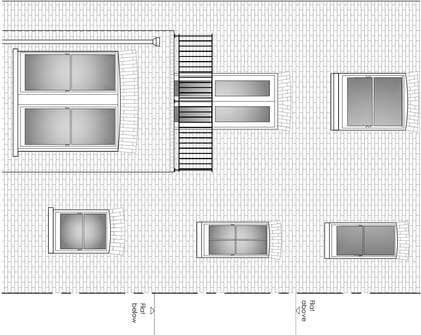
Proposed Elevation
