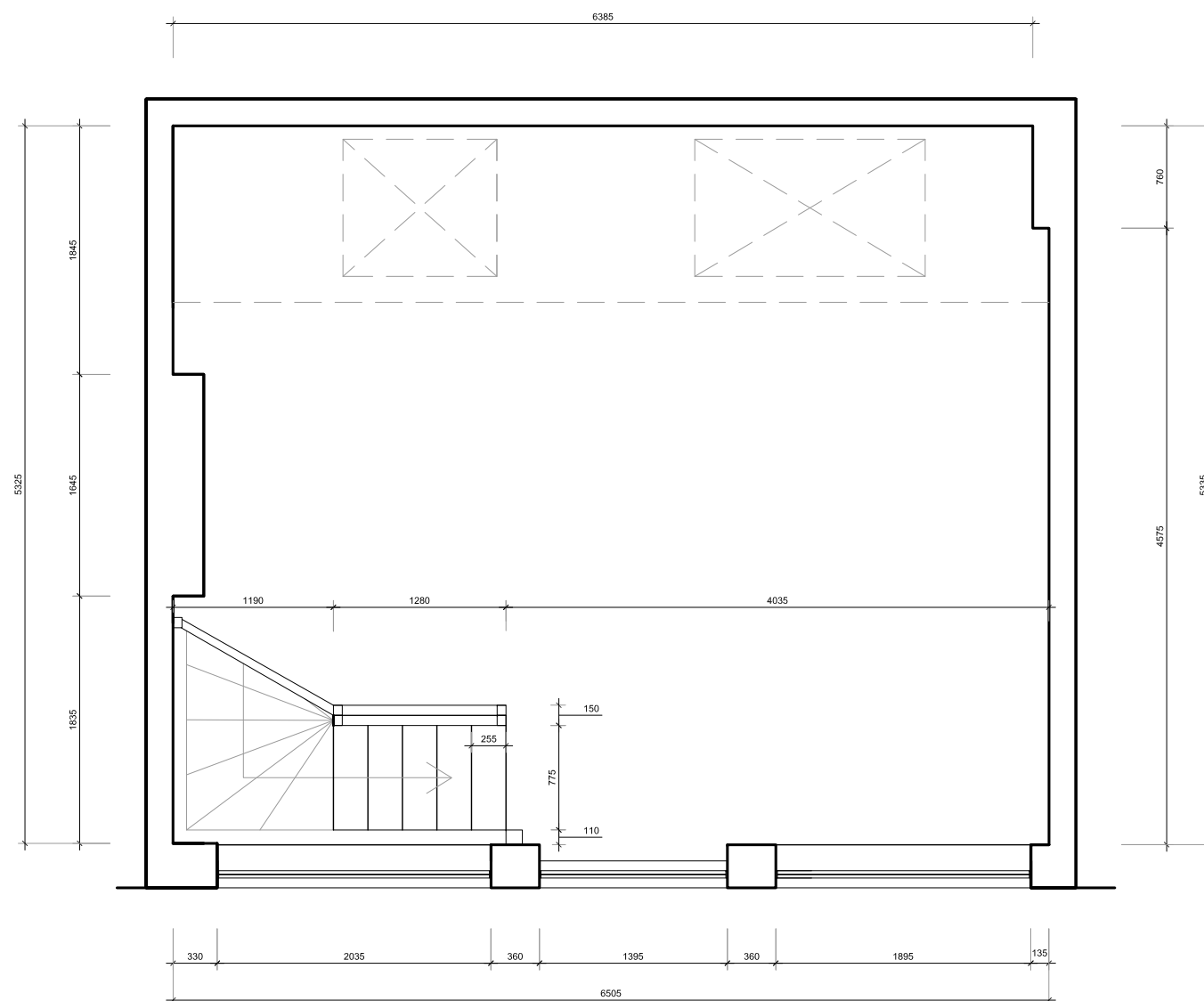
A FLOOR PLAN - SECOND FLOOR - EXISTING 1:50 @A3
