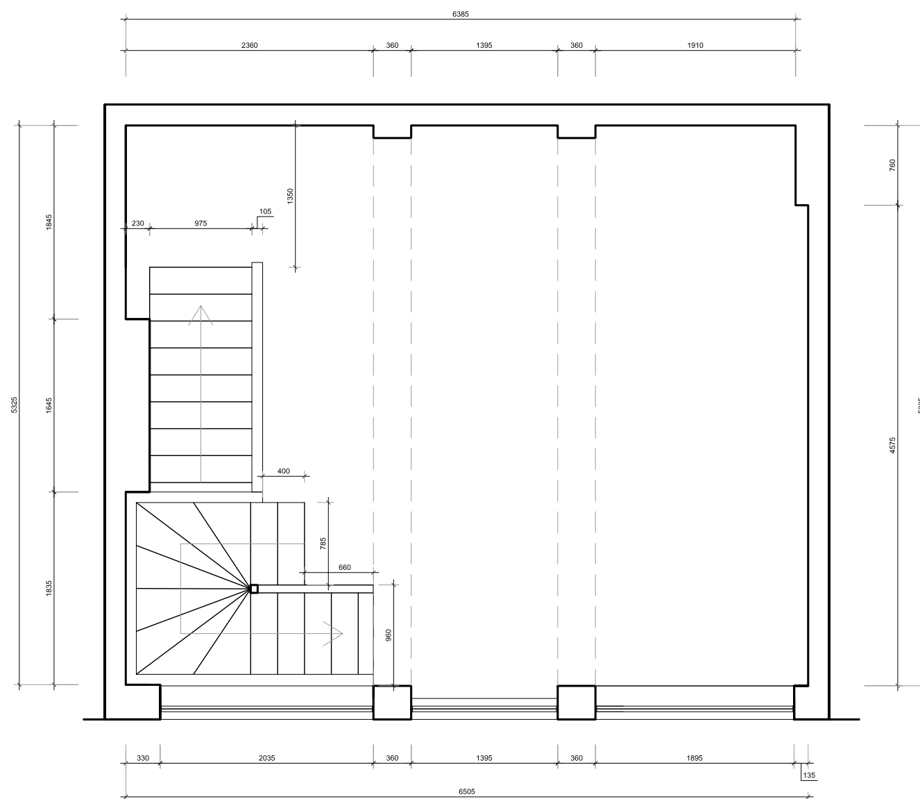
A FLOOR PLAN - FIRST FLOOR - EXISTING 1:50 @A3
