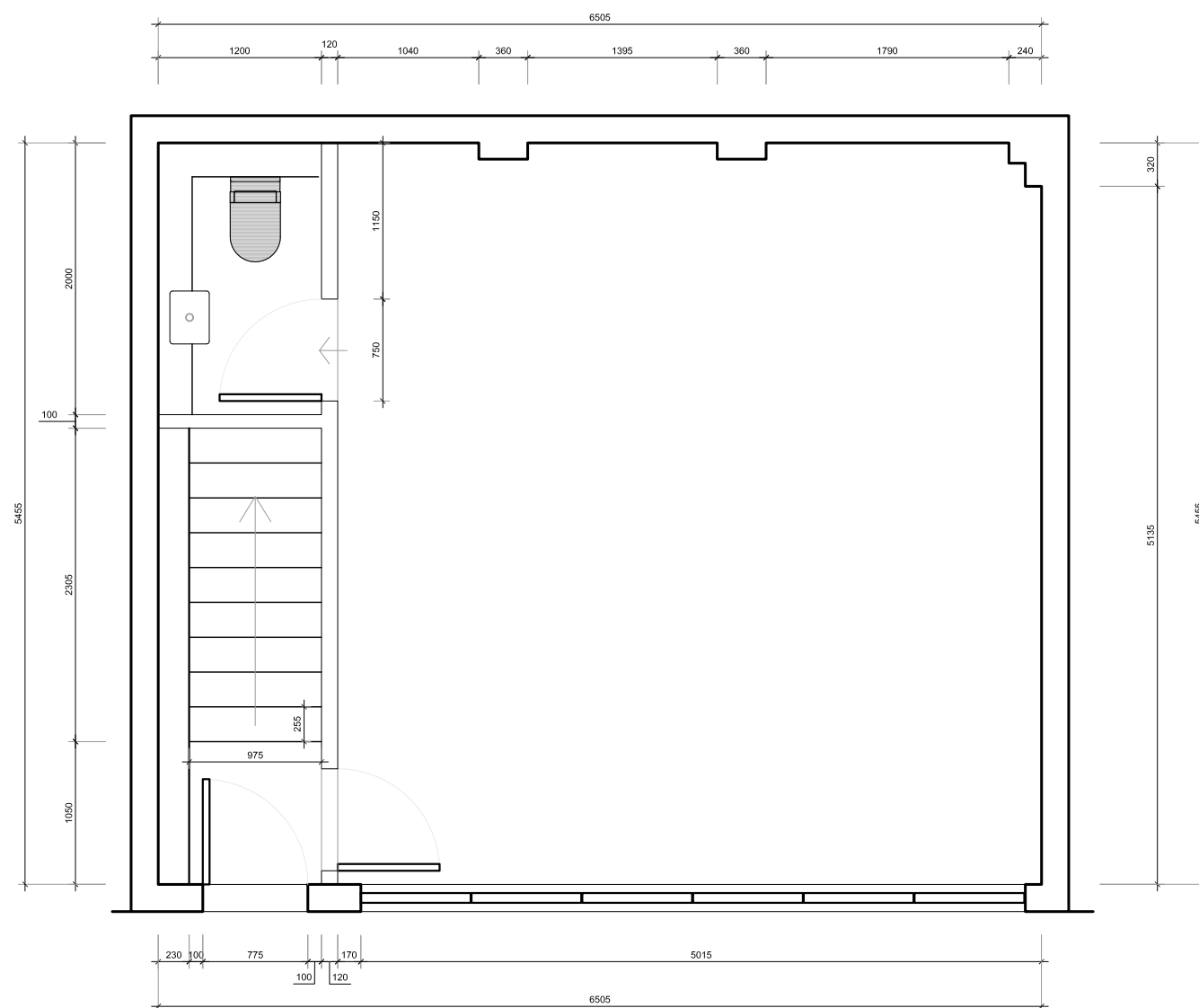
A FLOOR PLAN - GROUND FLOOR - EXISTING 1:50 @A3
