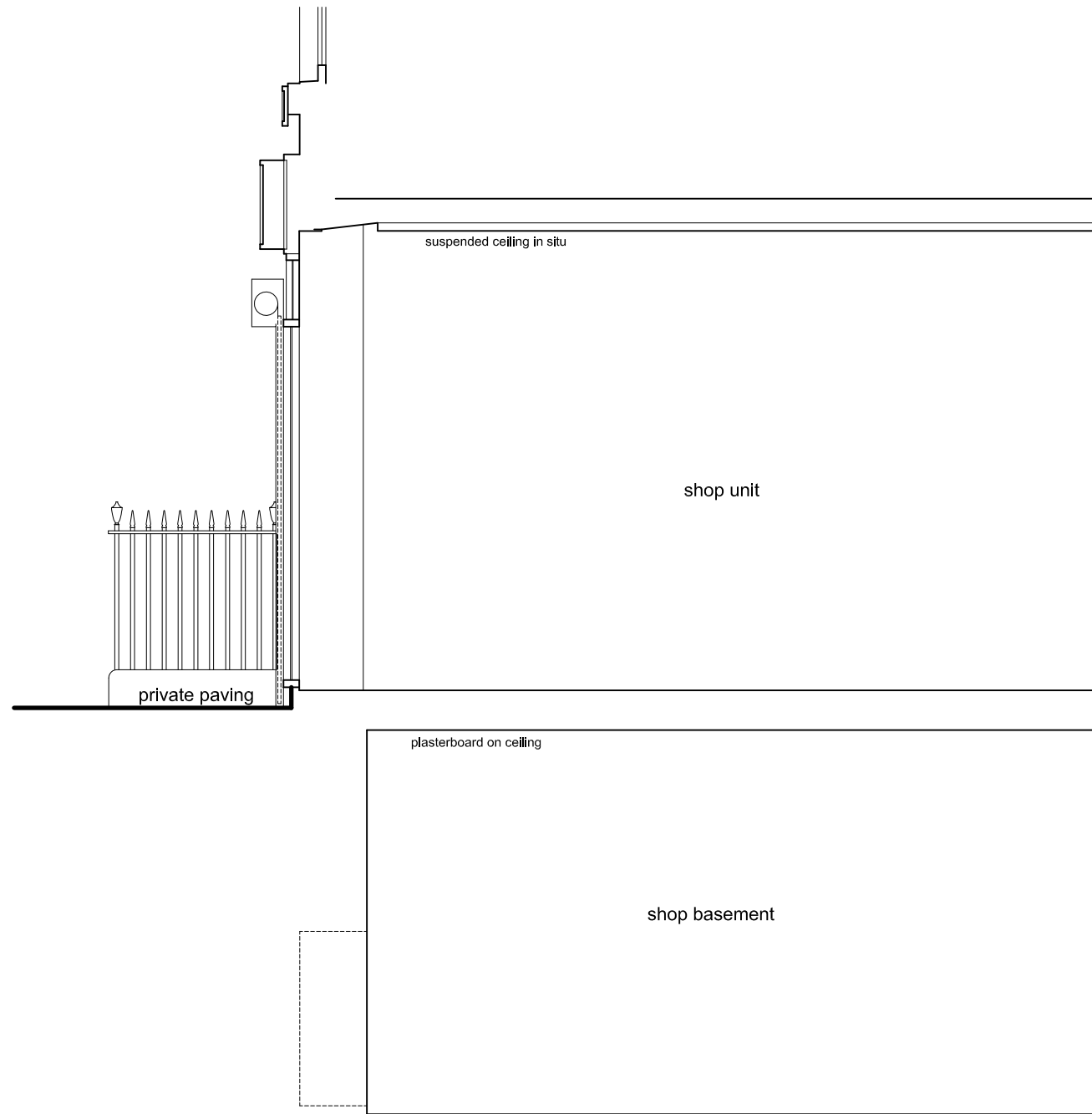
SECTION 0 1m
