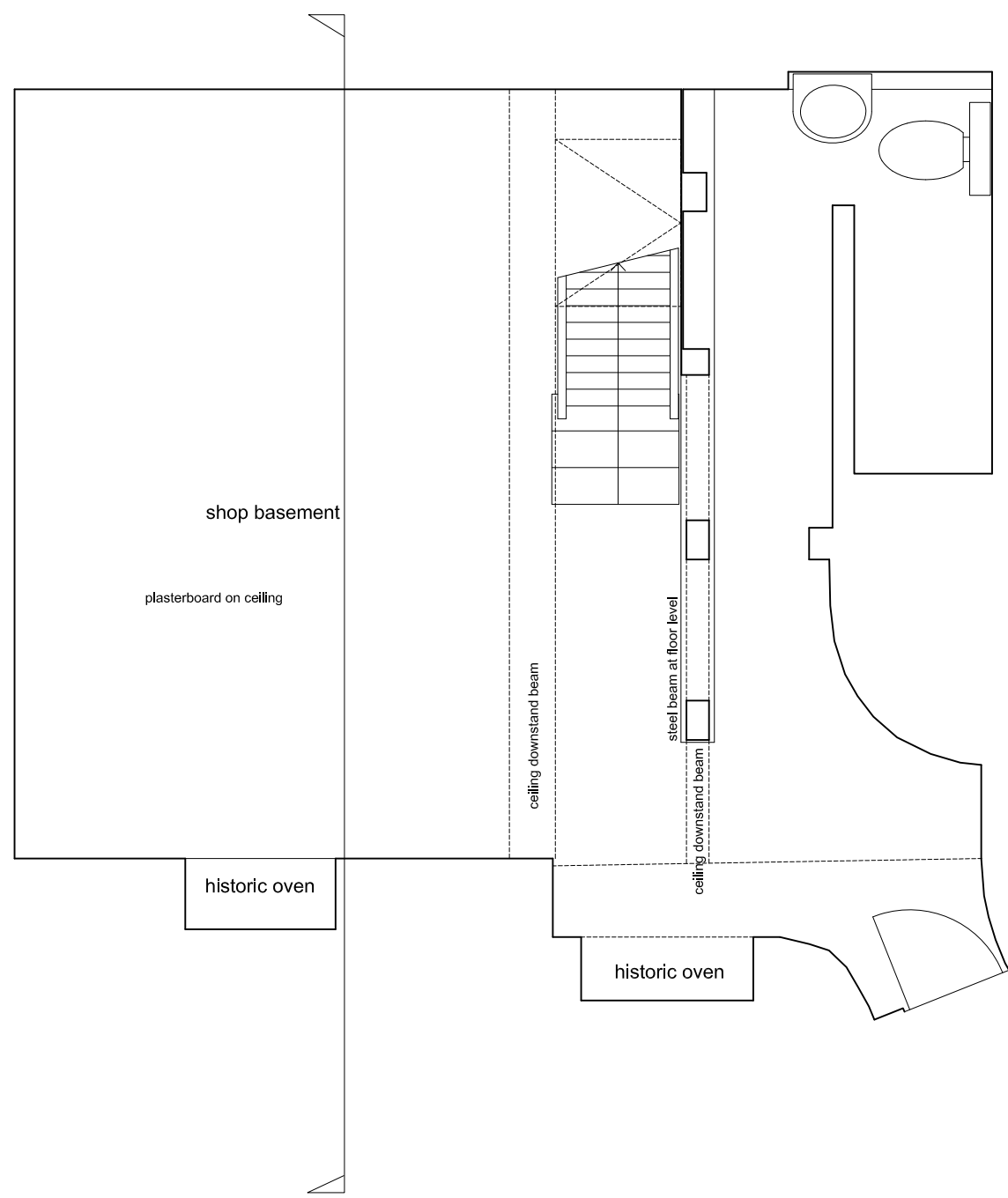
BASEMENT PLAN
