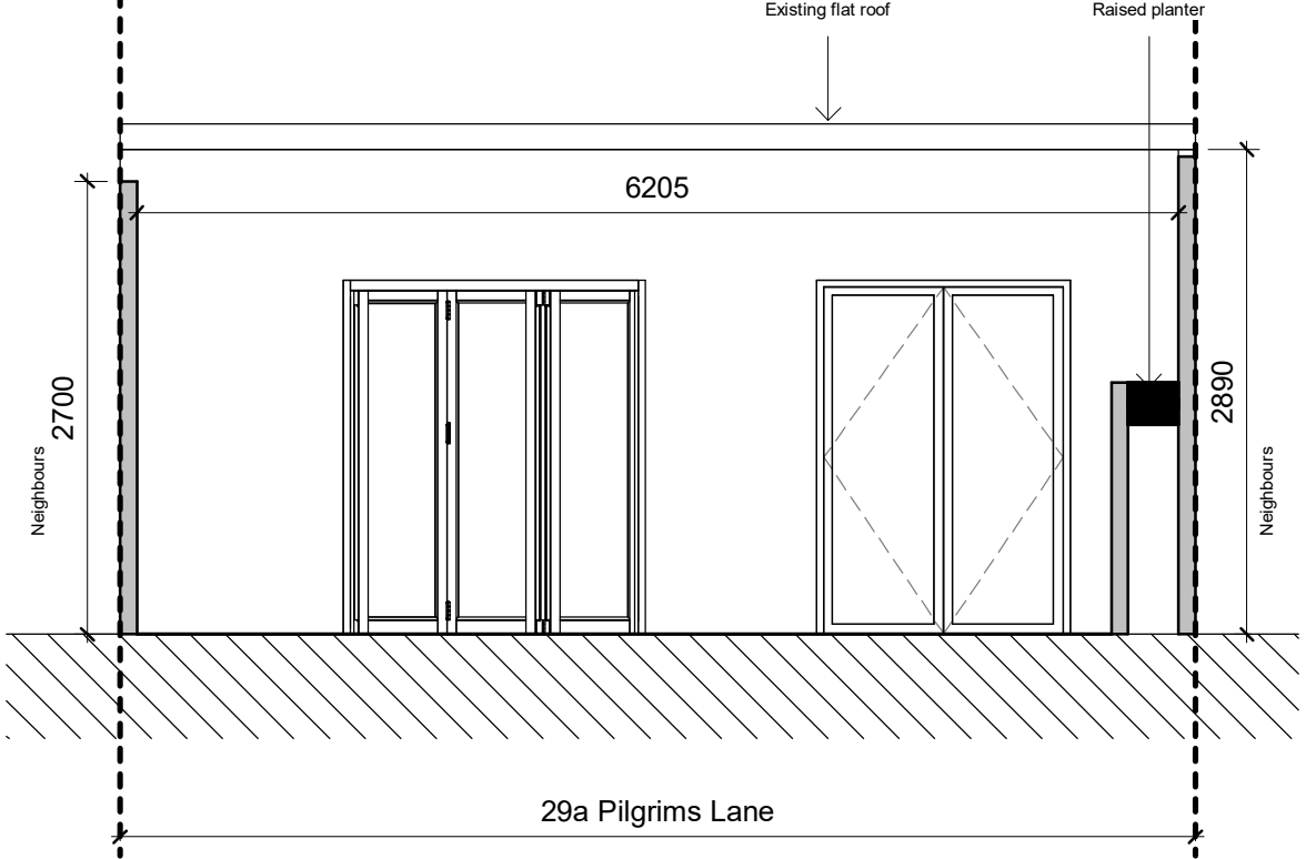
2 North West Elevation 1 : 50
