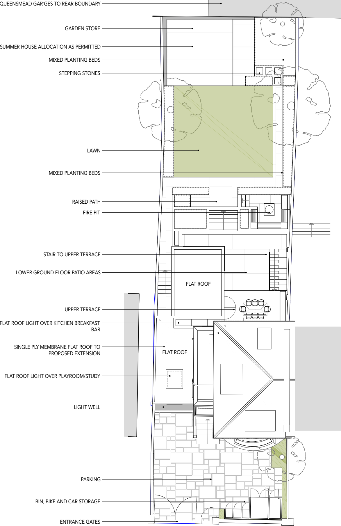
INDICATIVE SUMMER HOUSE AREA 1:100
