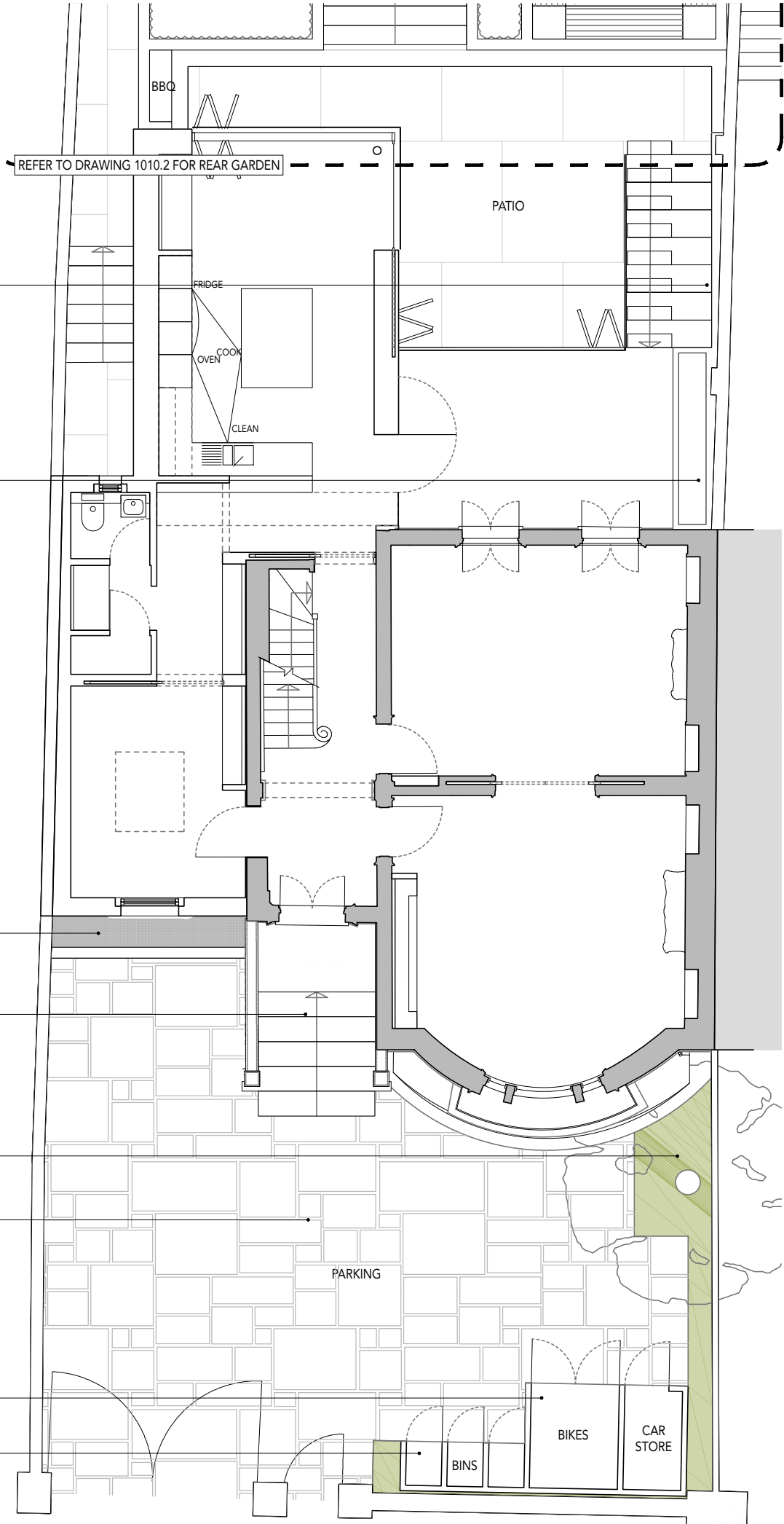
PROPOSED FRONT COURTYARD AND UPPER GROUND FLOOR PLAN 1:100
