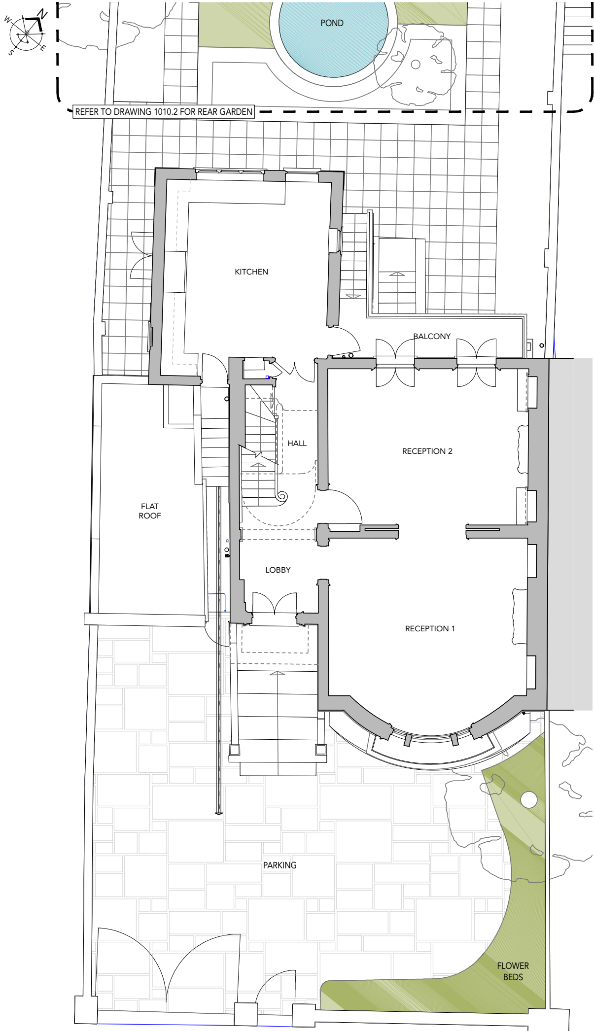
EXISTING FRONT COURTYARD AND UPPER GROUND FLOOR PLAN 1:100
