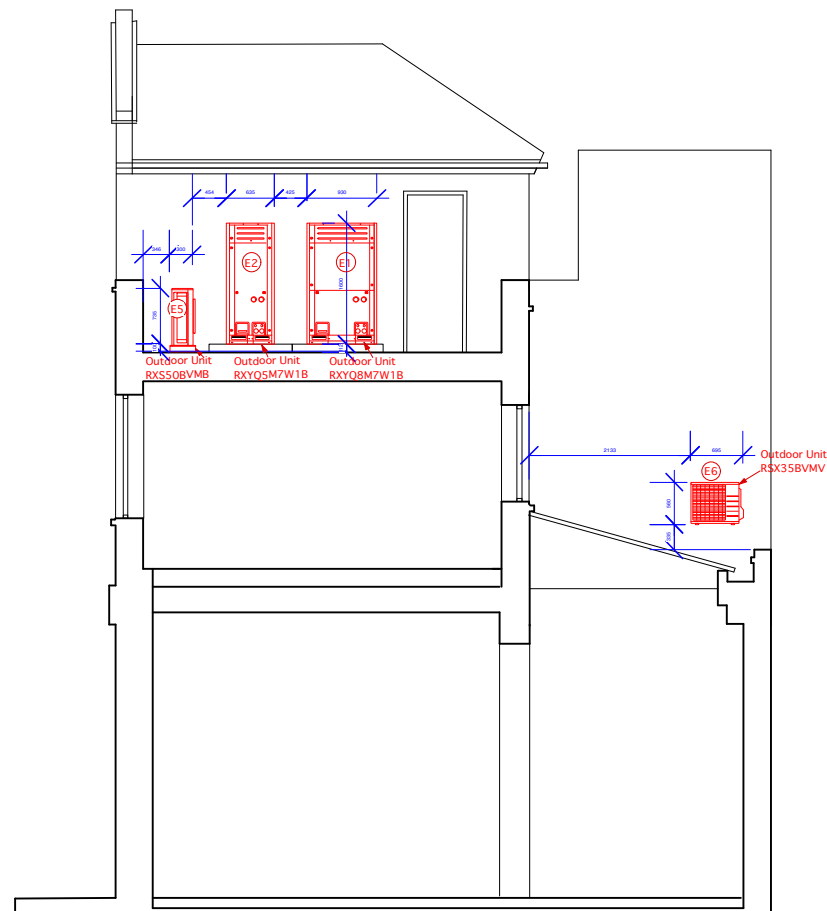
SECTION B-B
