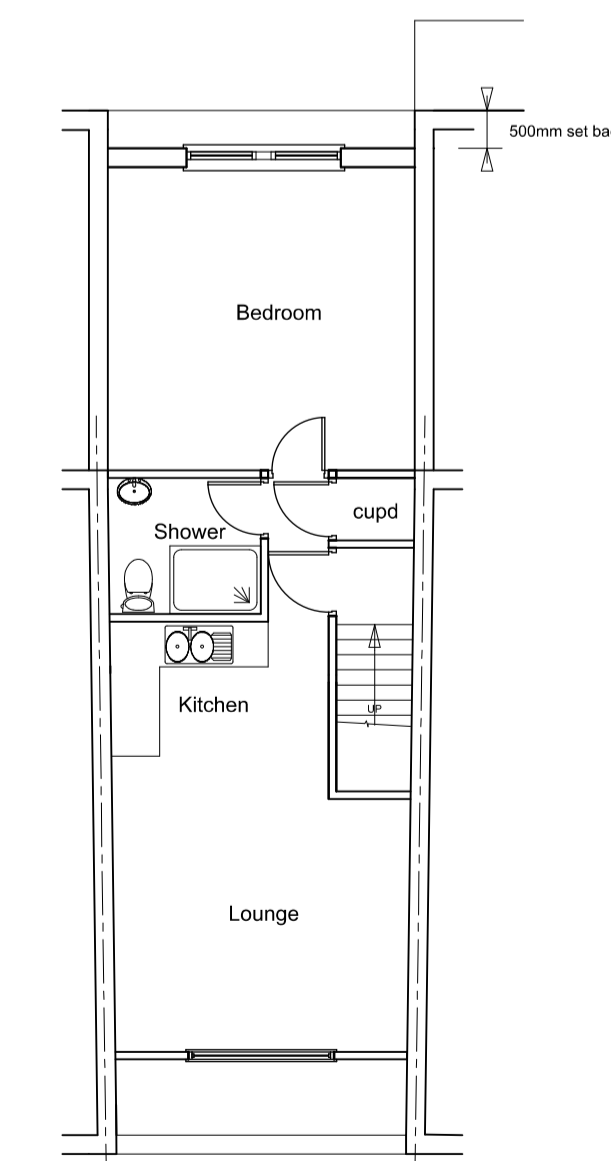
THIRD FLOOR PLAN (PROPOSED)
