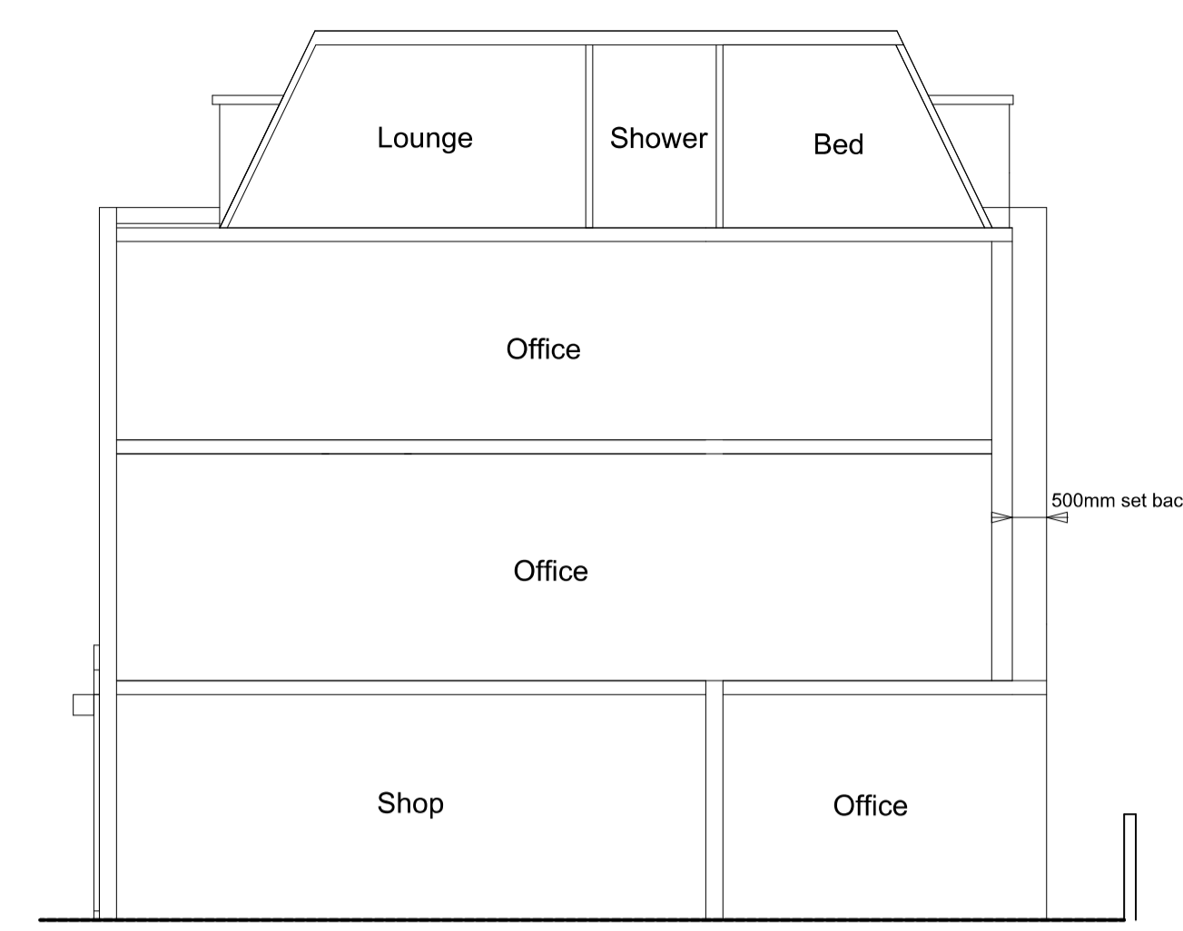
SECTION (PROPOSED)
