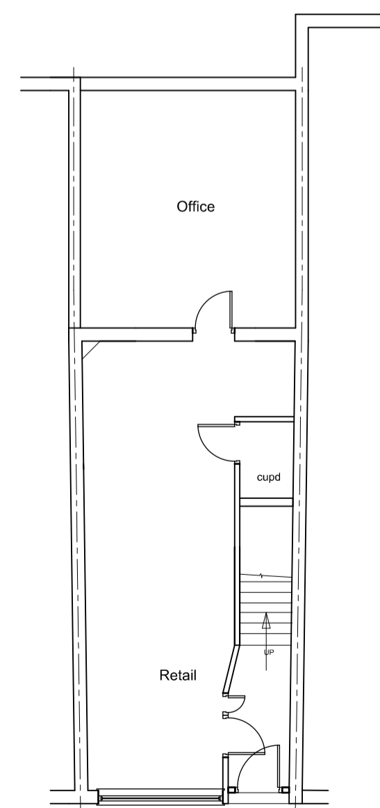
GROUND FLOOR PLAN (PROPOSED)
