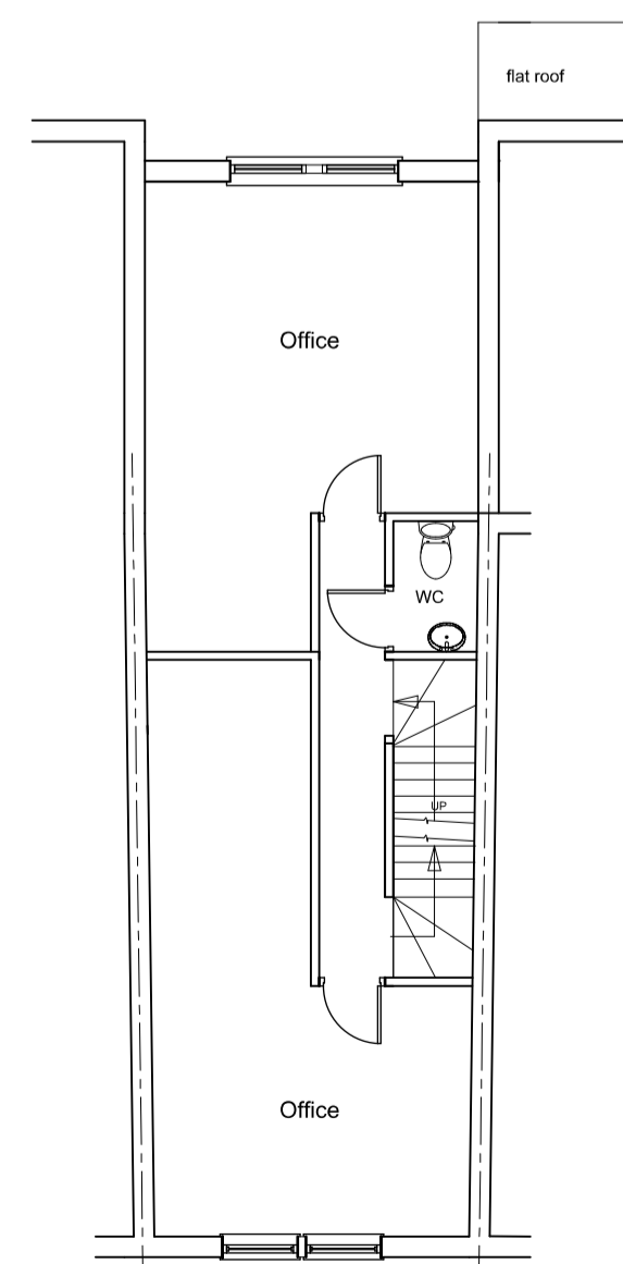
FIRST FLOOR PLAN (PROPOSED)
