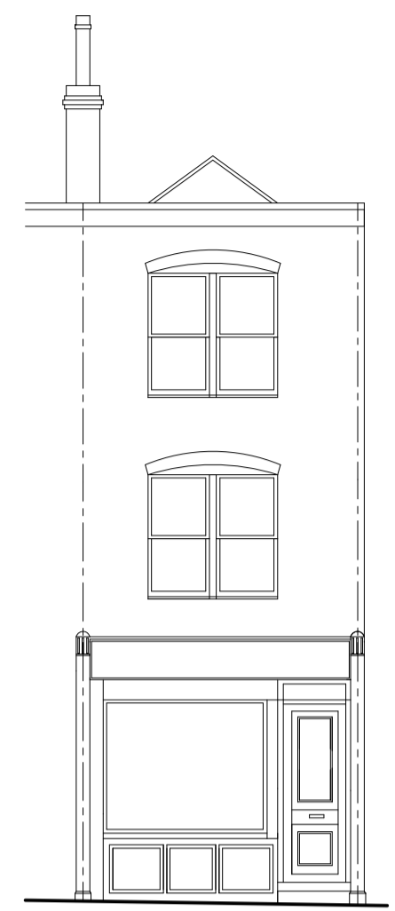
FRONT ELEVATION (EXISTING)
