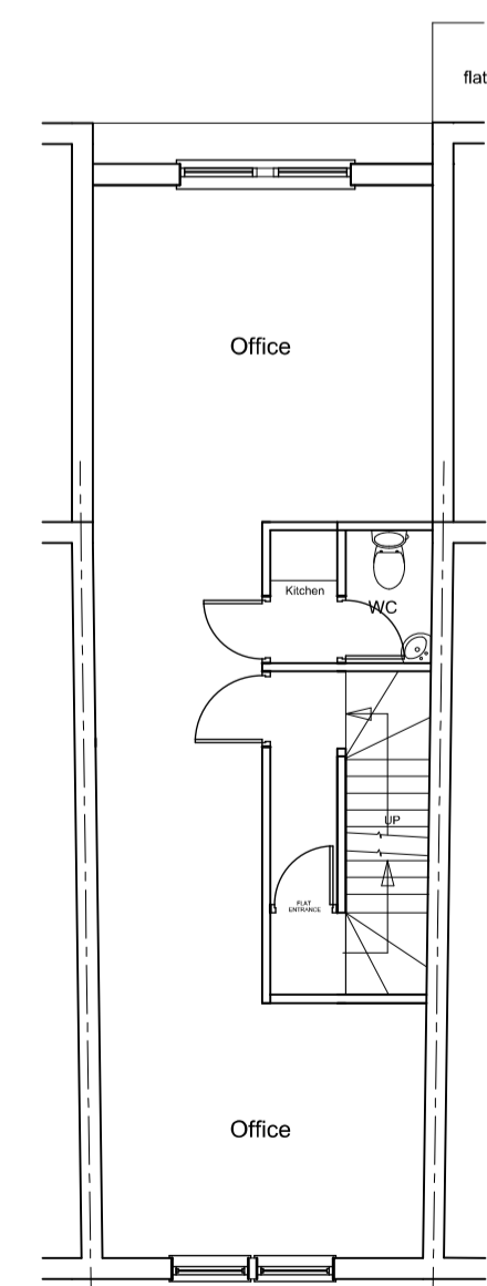
SECOND FLOOR PLAN (PROPOSED)
