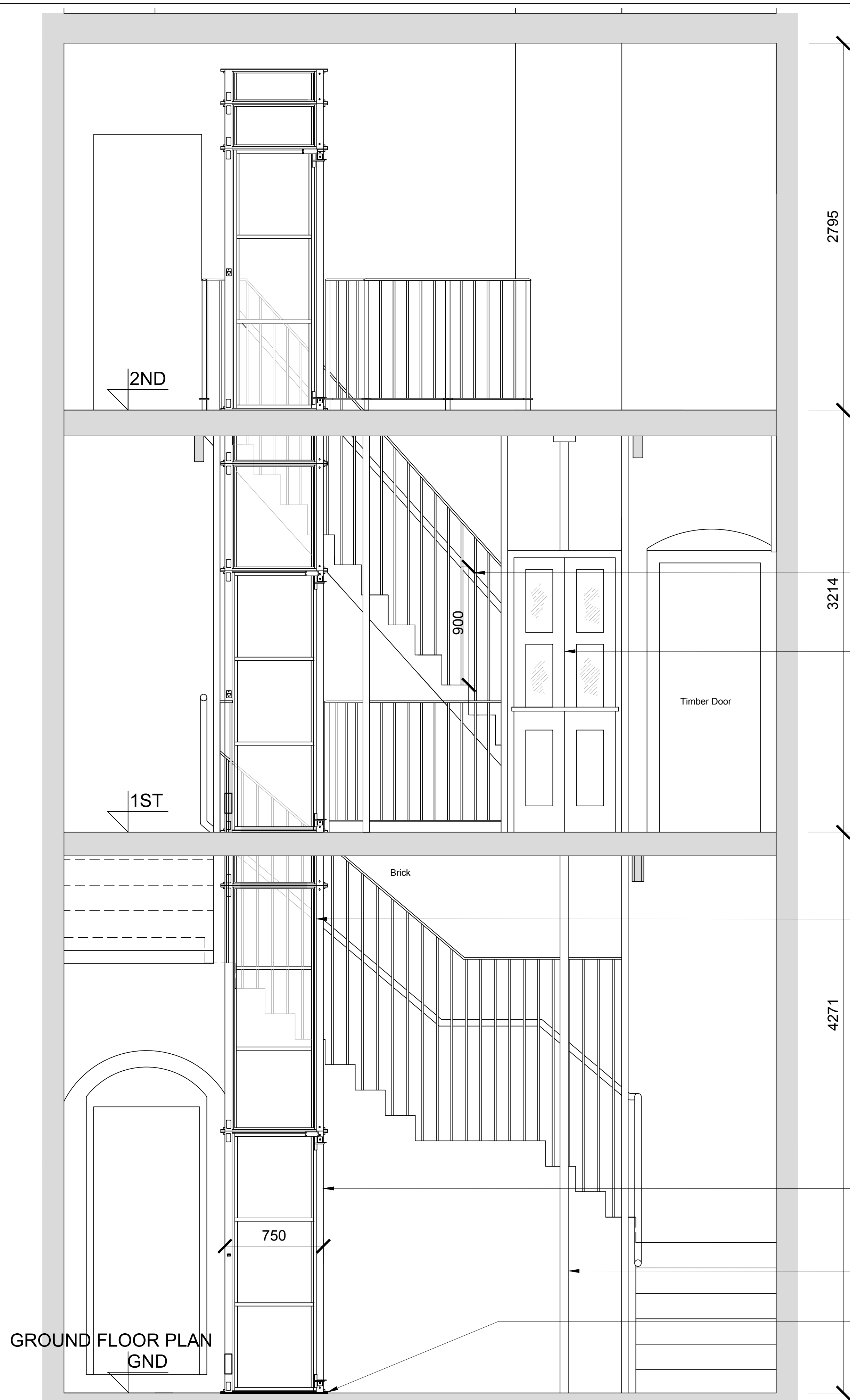
1 - NORTH LIFT ELEVATION
