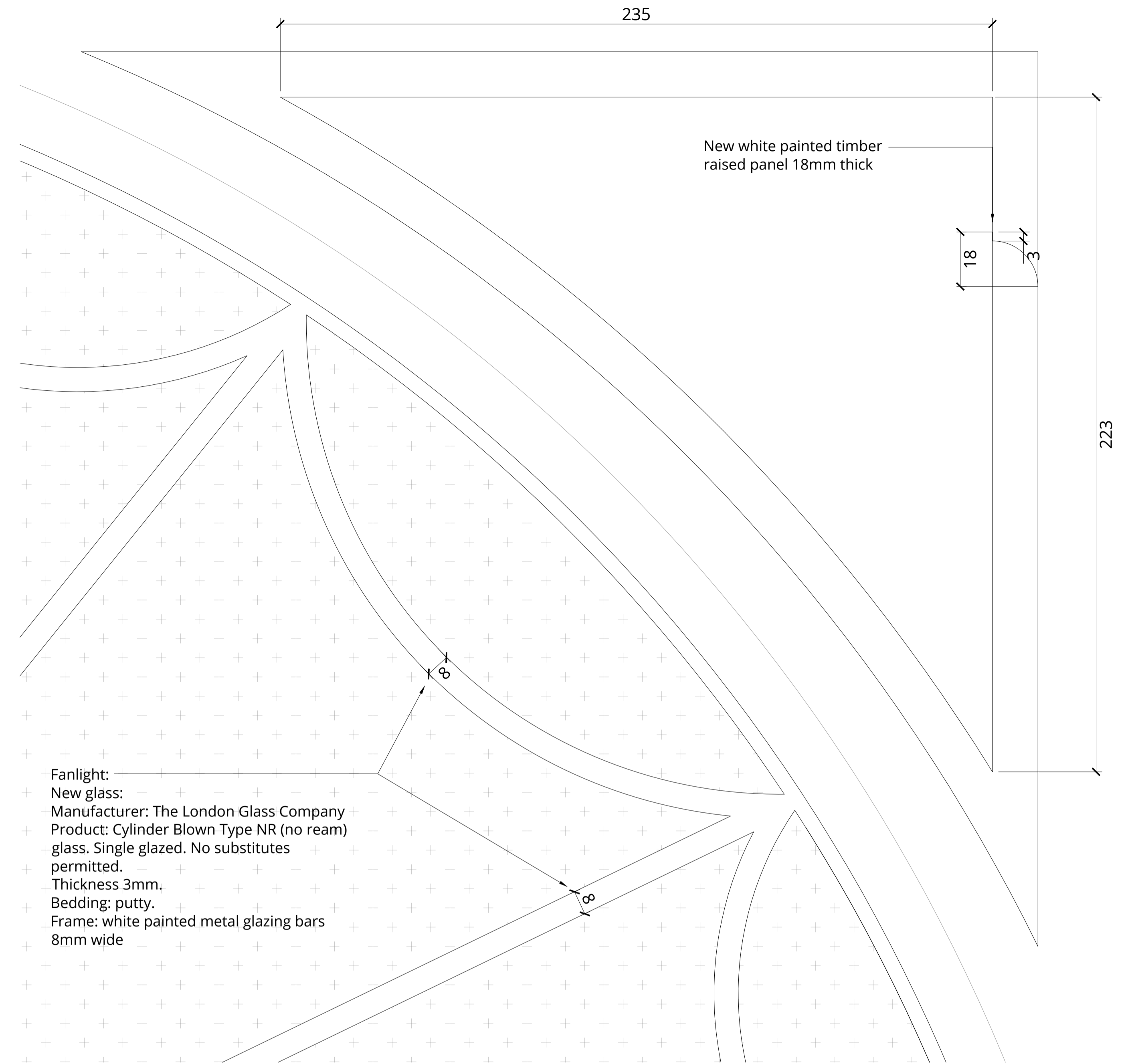
02 819 PROPOSED ELEVATION DETAIL FANLIGHT 1:1@A1
