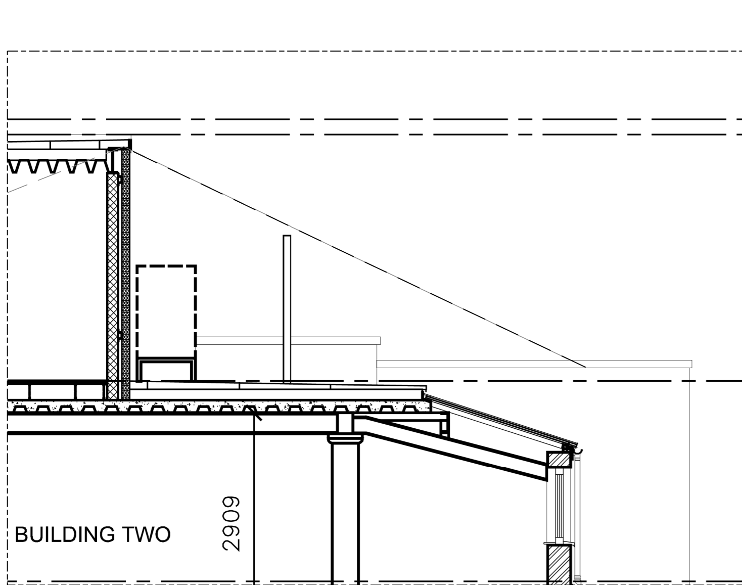
Extract from PKS Architects drawing 020-05 Rev A
