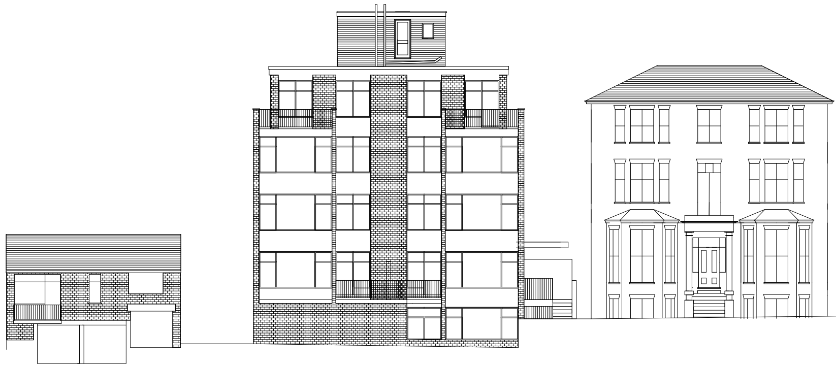
FRONT ELEVATION
