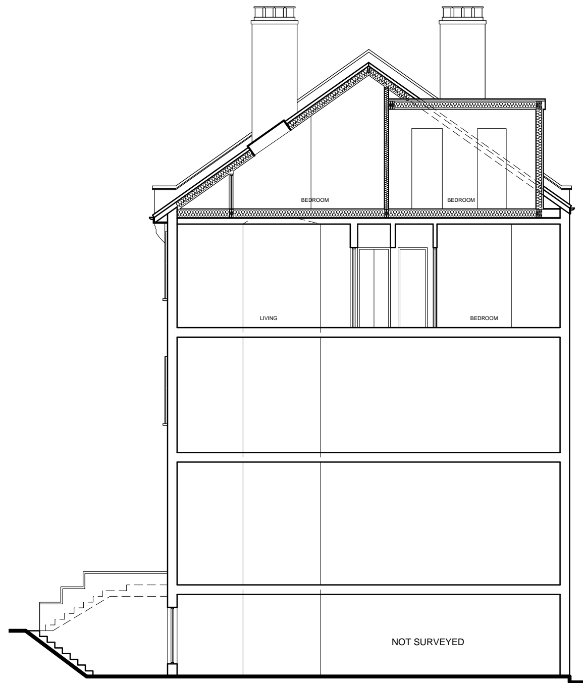
Section C-C
