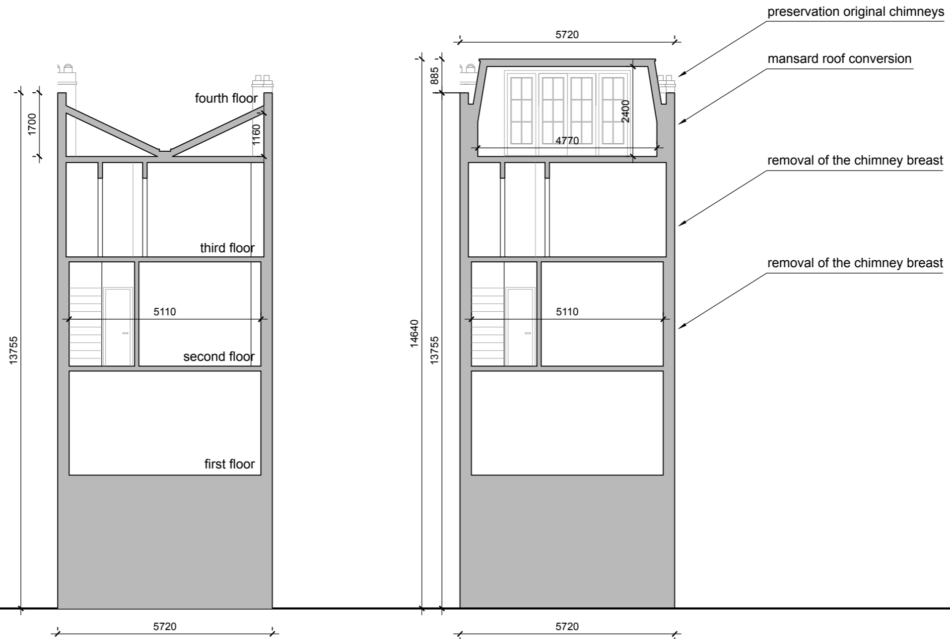
EXISTING SITUATION_CROSS SECTION 44 FALKLAND ROAD
