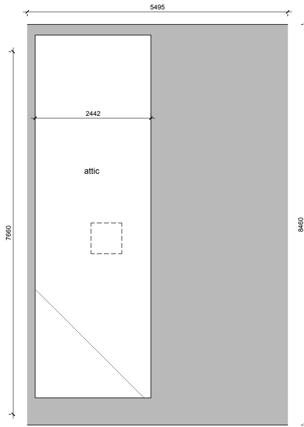
EXISTING SITUATION_FOURTH FLOOR_ATTIC FLAT 44c
