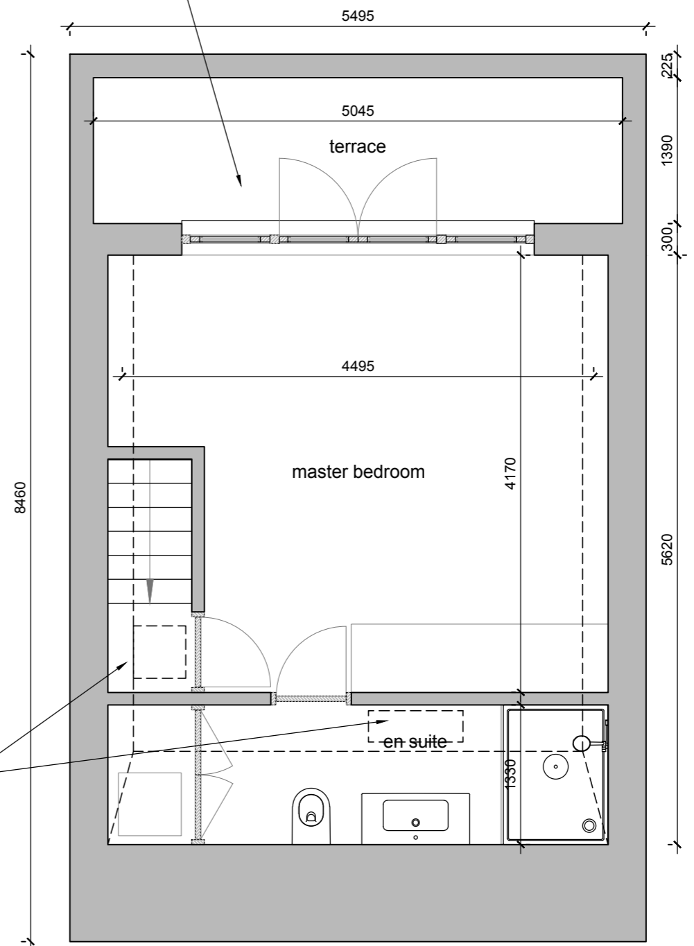
DESIGN PROPOSAL MANSARD ROOF_FOURTH FLOOR_FLOORPLAN FLAT 44c
