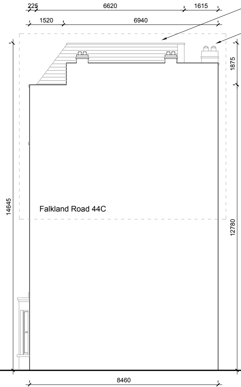
DESIGN PROPOSAL_SIDE ELEVATION 44 FALKLAND ROAD
