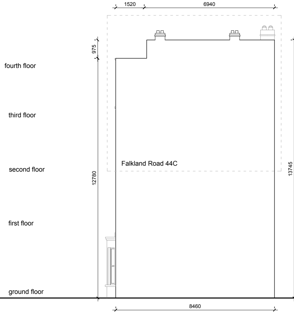
EXISTING SITUATION_SIDE ELEVATION 44 FALKLAND ROAD
