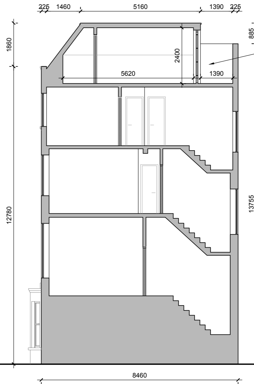
DESIGN PROPOSAL _LONGITUDINAL SECTION 44 FALKLAND ROAD
