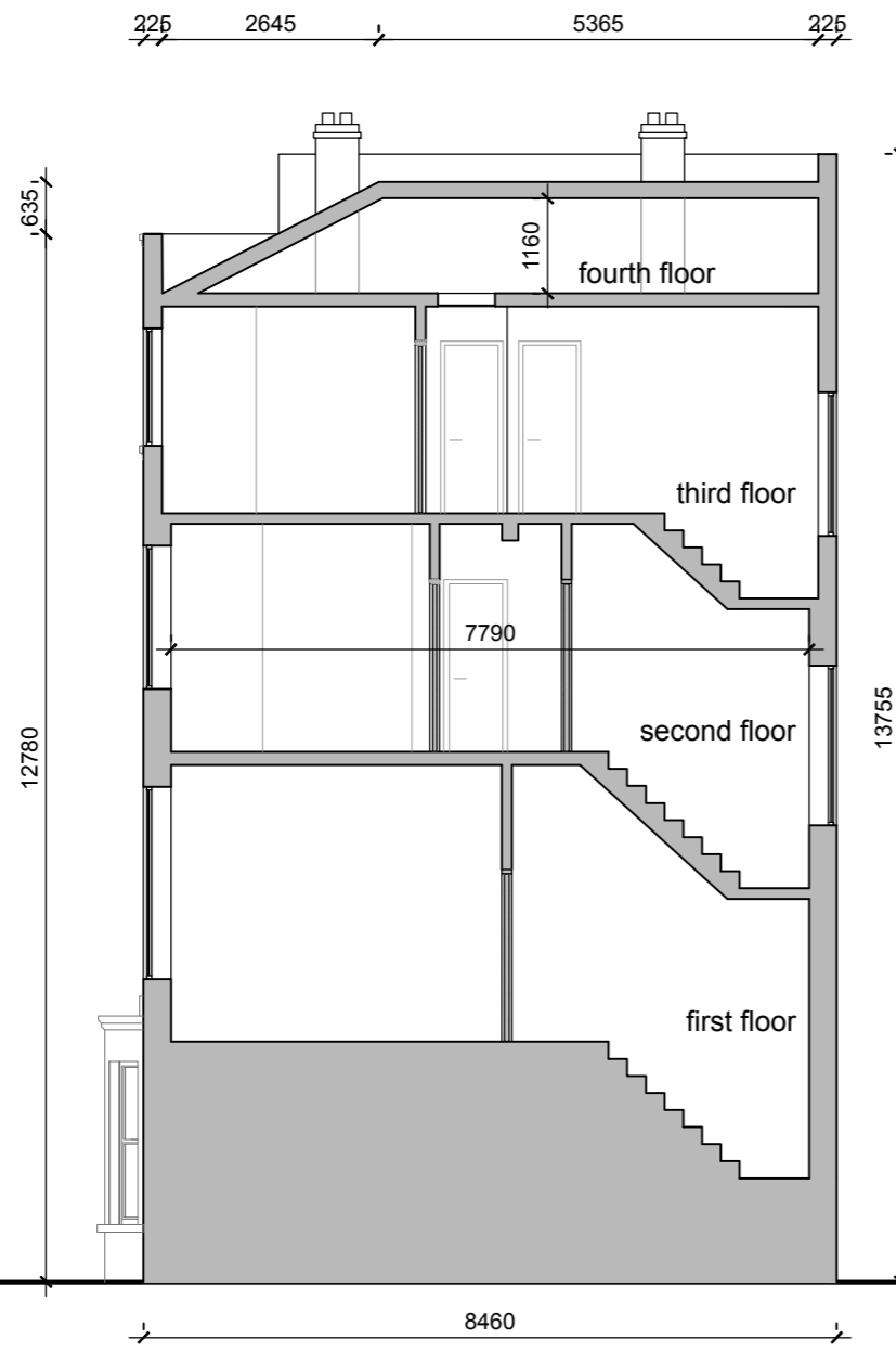
EXISTING SITUATION _LONGITUDINAL SECTION 44 FALKLAND ROAD
