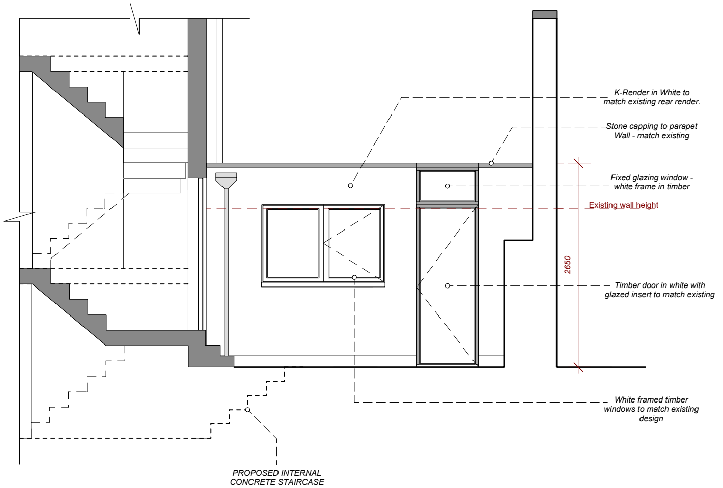
PROPOSED ELEVATION 3
