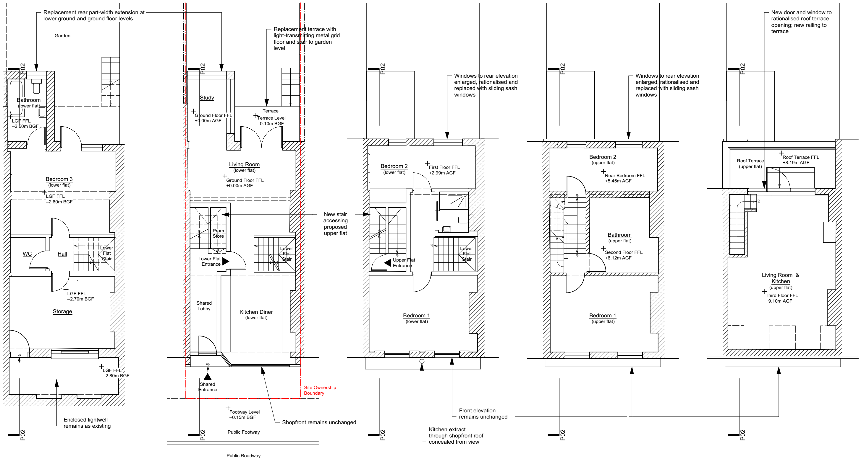
Lower Ground Floor Plan Proposed
