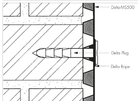
Figure 2 Delta Plug fixing detail
