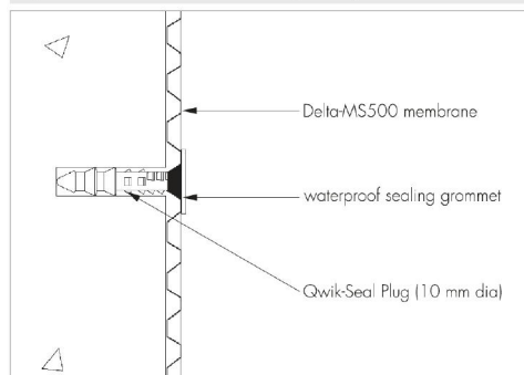
Figure 1 Delta Qwik-Seal Plug fixing detail
