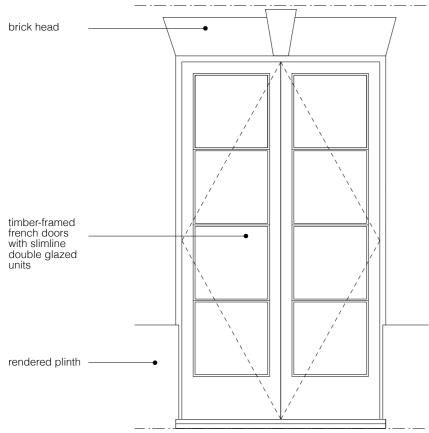
BASEMENT FRONT WINDOW ELEVATION AS PROPOSED
