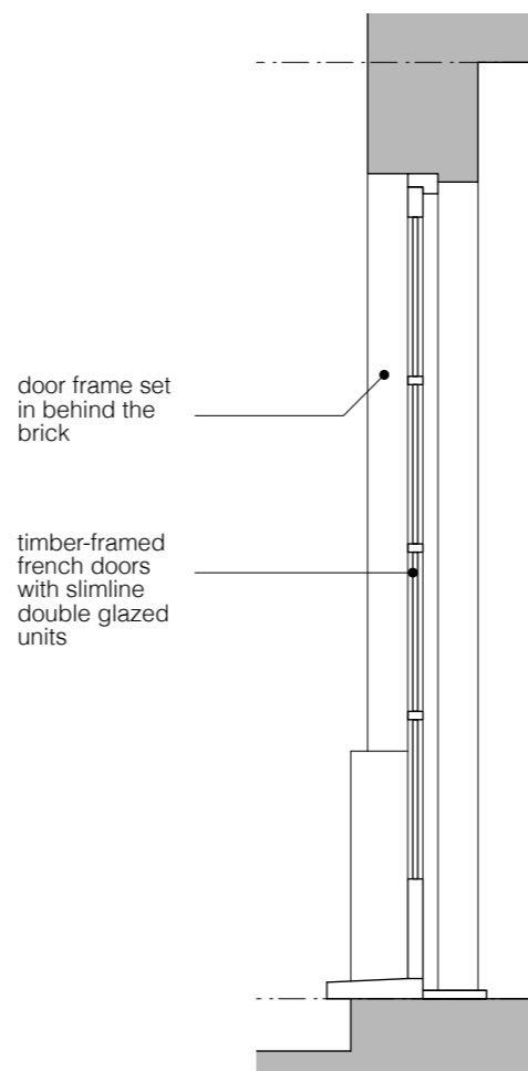
BASEMENT FRONT WINDOW SECTION AS PROPOSED
