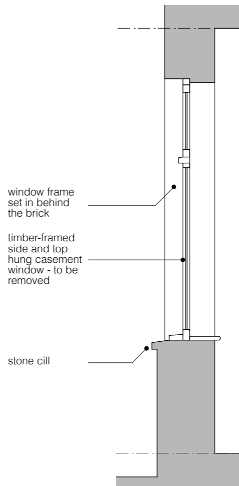
BASEMENT FRONT WINDOW SECTION AS EXISTING
