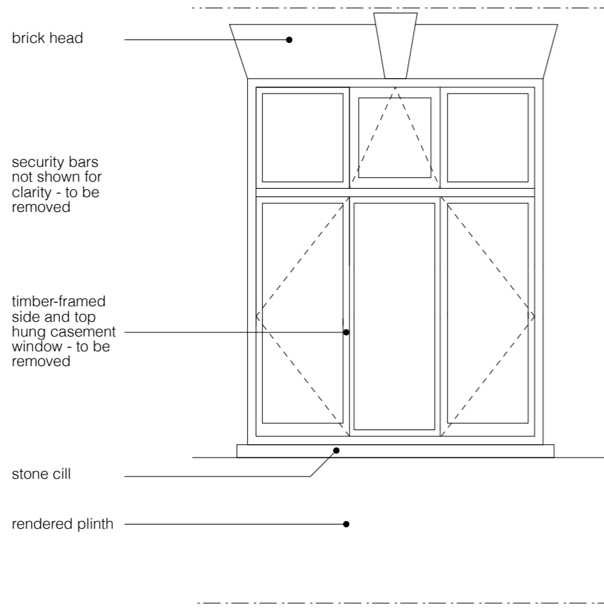
BASEMENT FRONT WINDOW ELEVATION AS EXISTING
