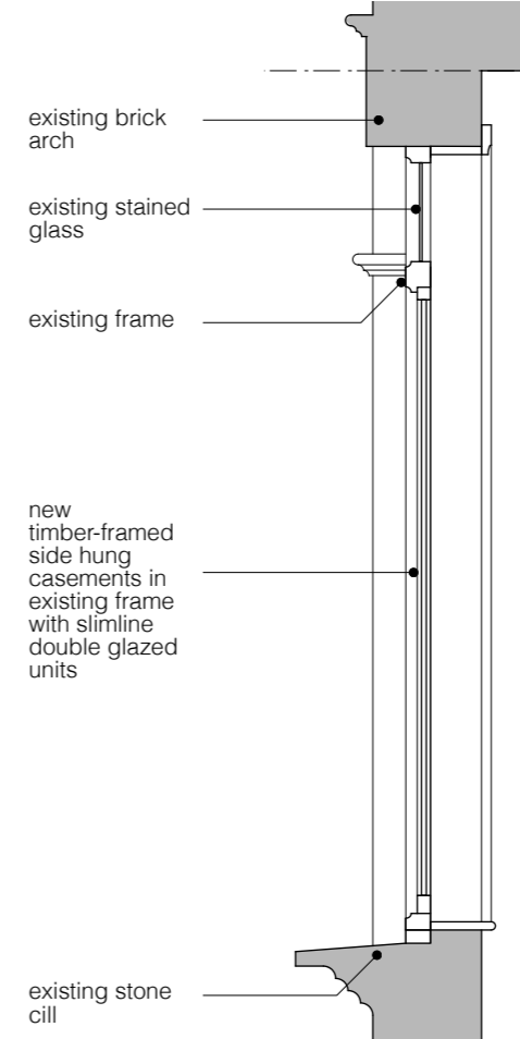
WINDOWS 1&2 SECTION AS PROPOSED
