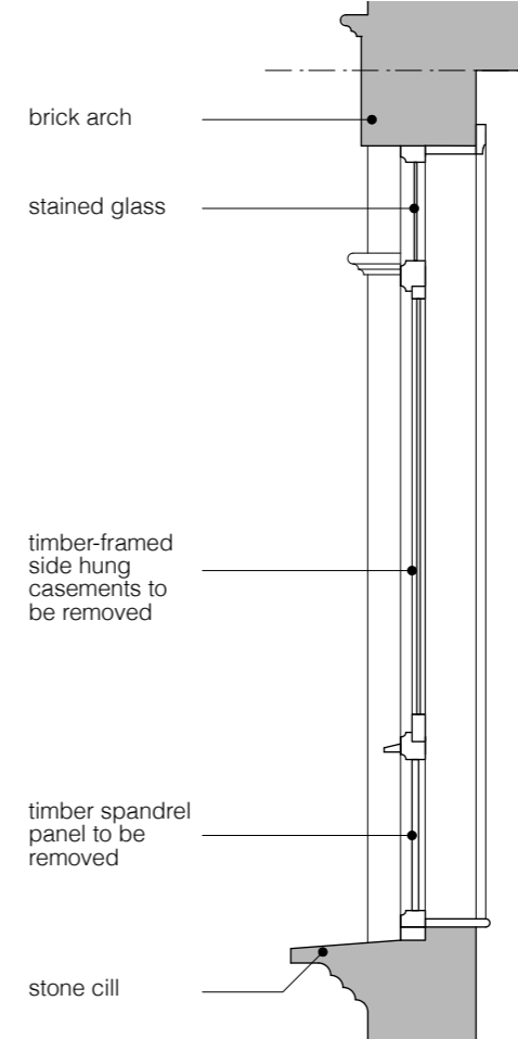
WINDOWS 1&2 SECTION AS EXISTING
