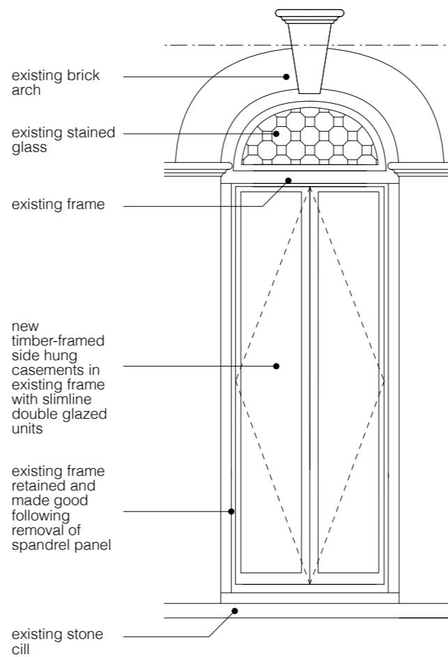
WINDOW 2 ELEVATION AS PROPOSED
