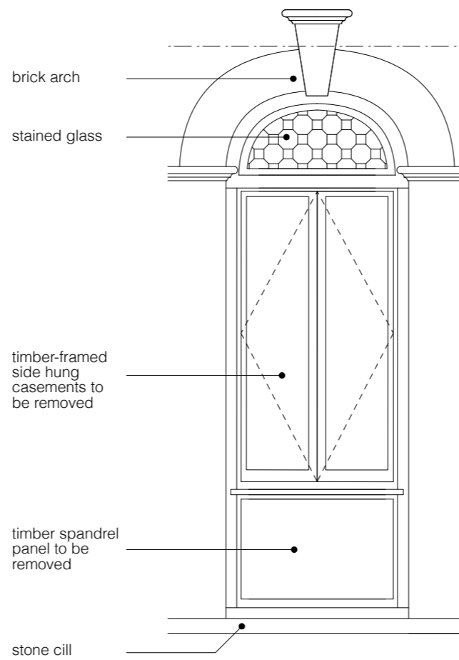
WINDOW 2 ELEVATION AS EXISTING
