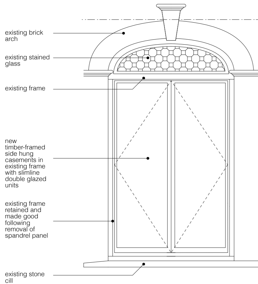
WINDOW 1 ELEVATION AS PROPOSED
