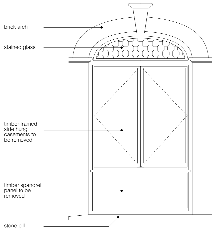
WINDOW 1 ELEVATION AS EXISTING
