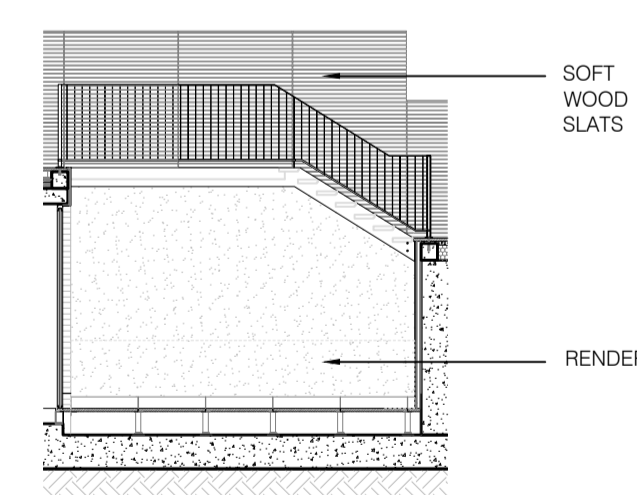
Elevation H Scale 1:100
