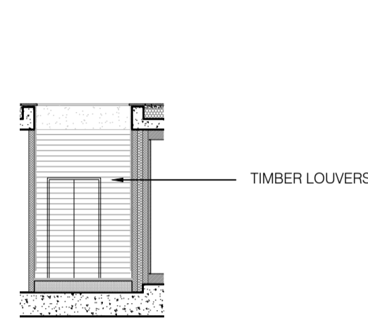
Elevation 1C Scale 1:100
