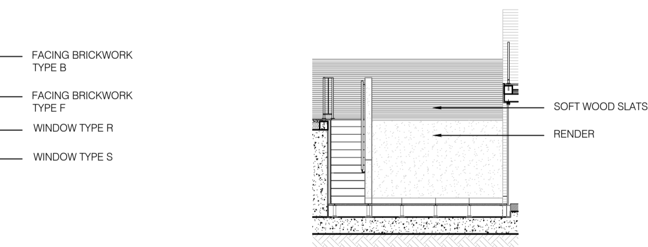
Elevation F Scale 1:100
