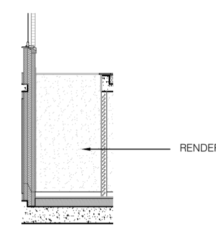
Elevation 2B Scale 1:100
