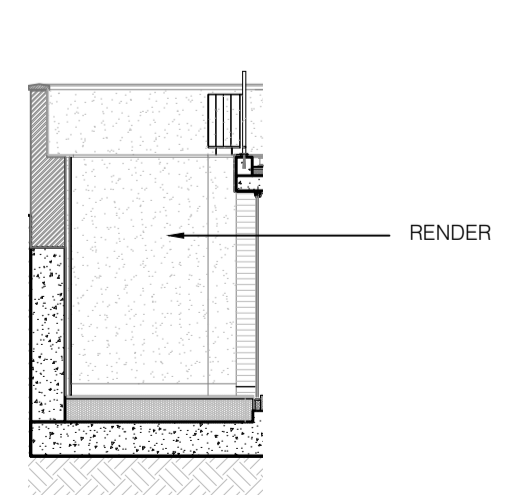
Elevation K Scale 1:100
