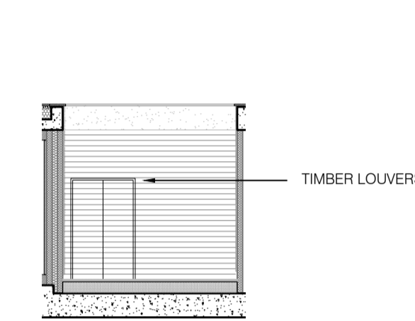
Elevation 2C Scale 1:100
