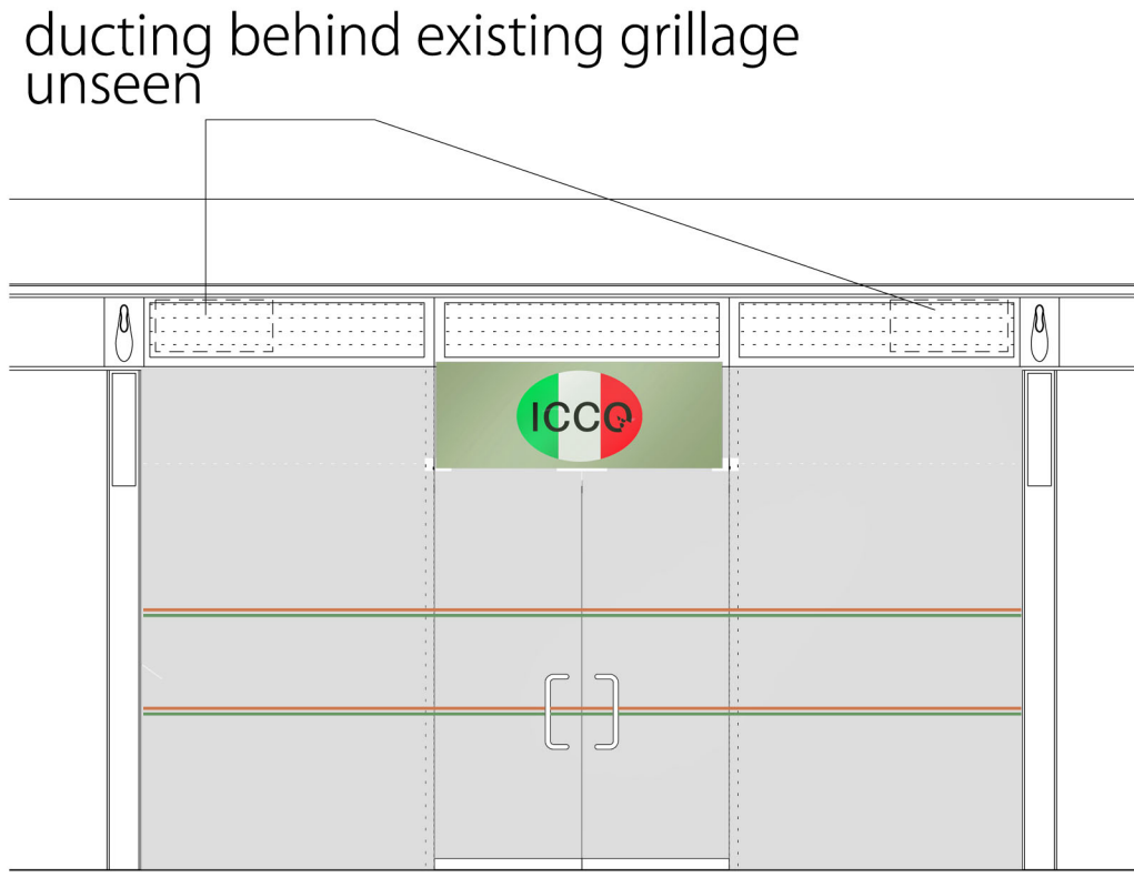
proposed front elevation behind canopy
