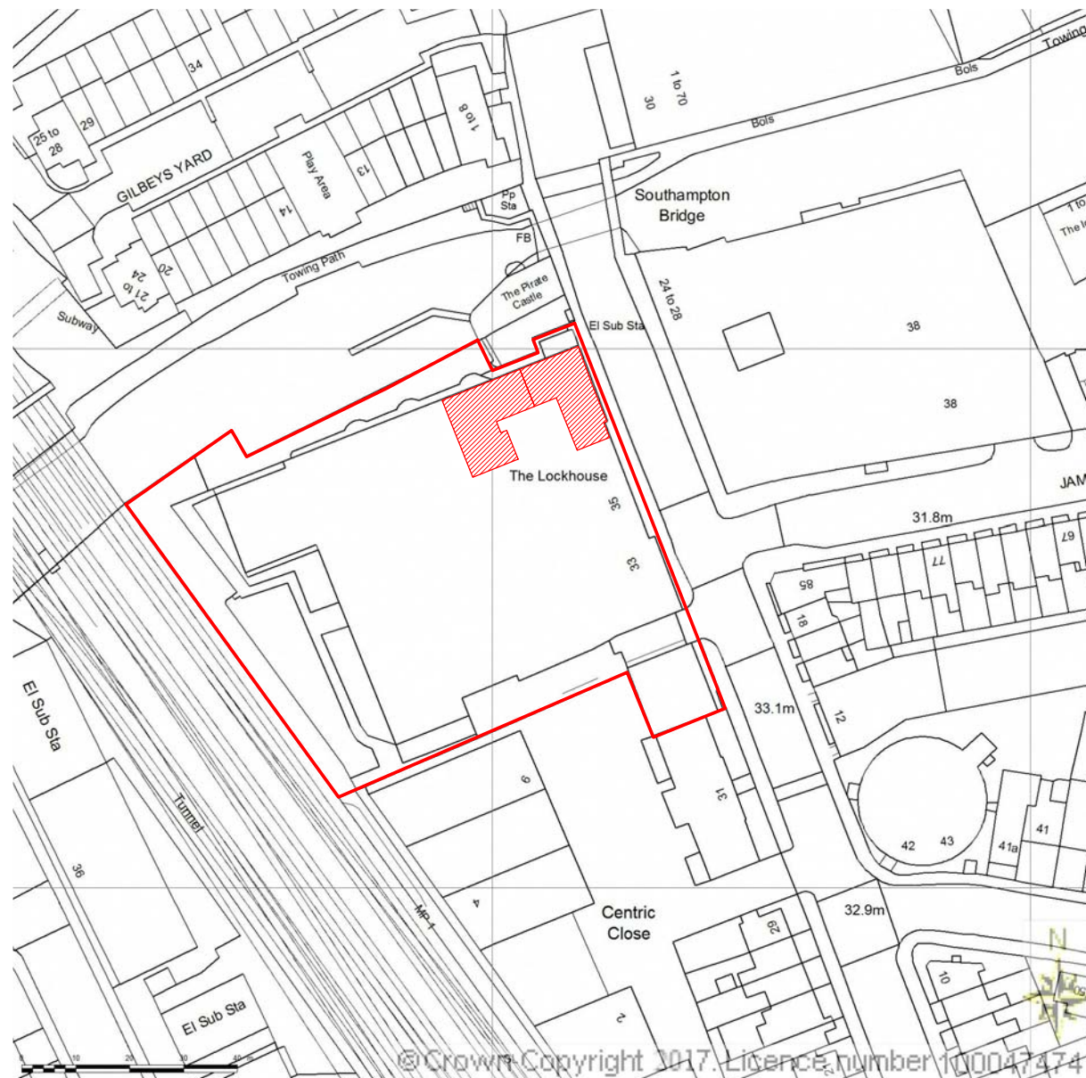
1 Location Plan 1 : 1250
