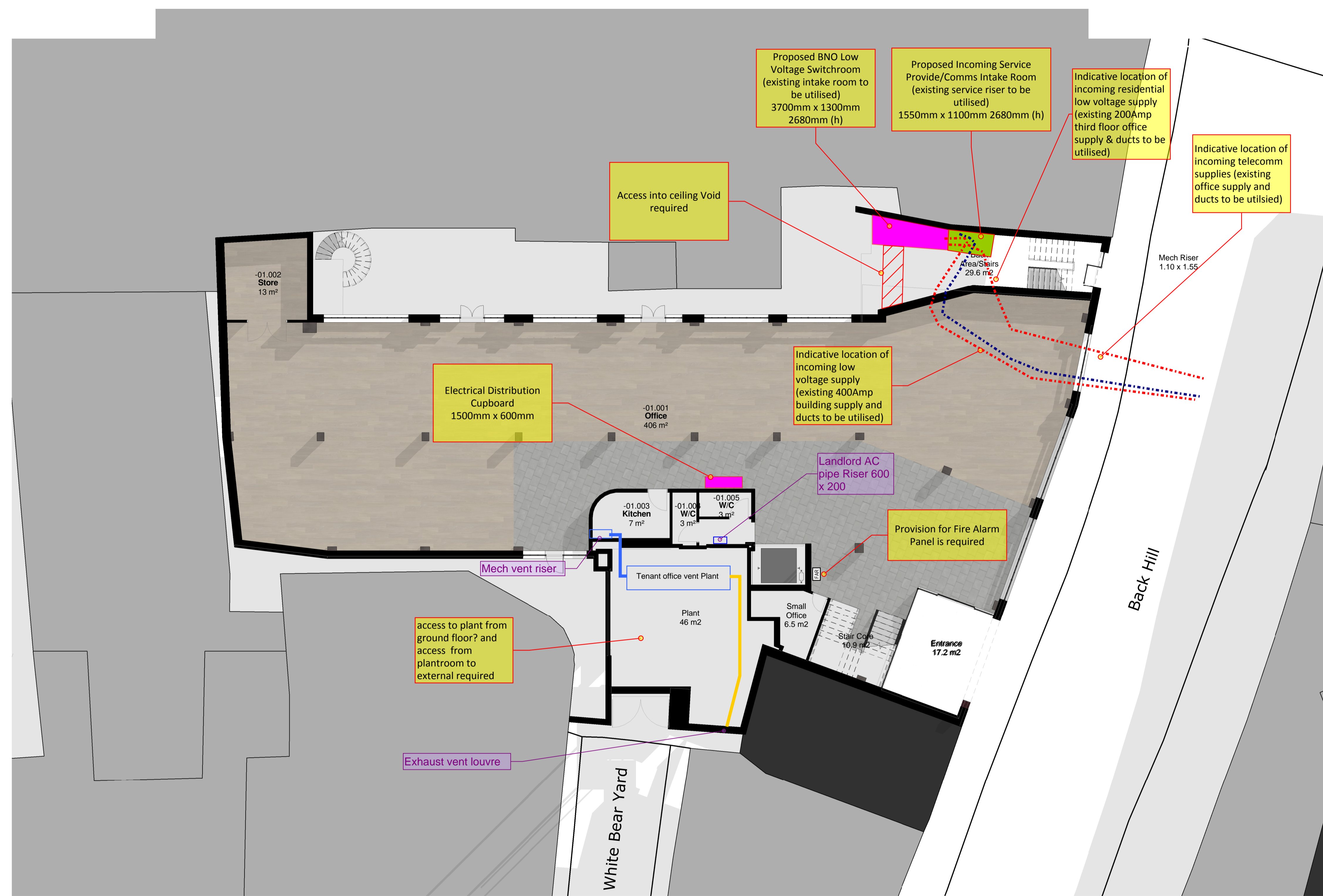
1 2000_B1-Lower Ground (Proposed) 1:100
