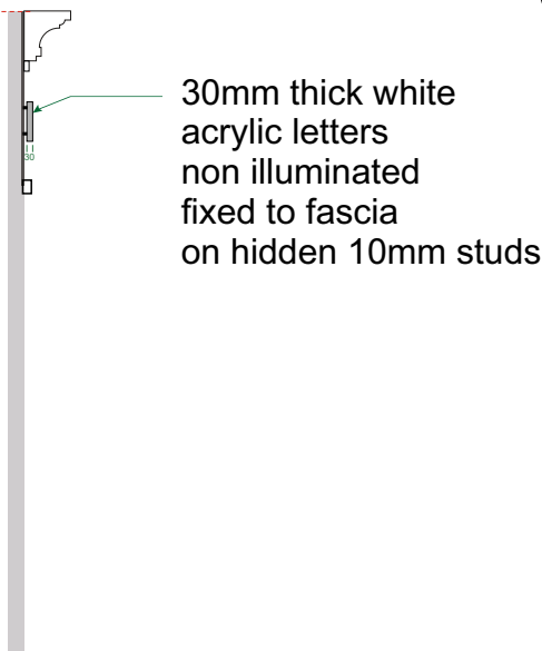
Side section view of fascia sign
