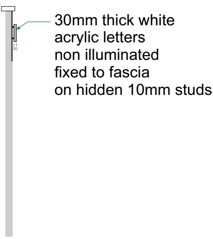
Side section view of fascia sign
