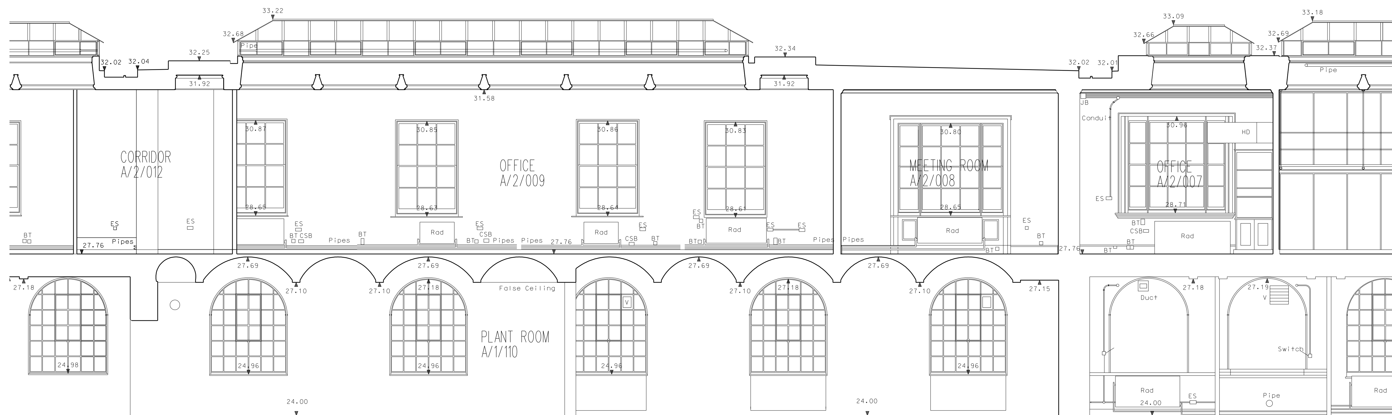
TYPICAL LONGITUDINAL SECTION AT SOUTH END
