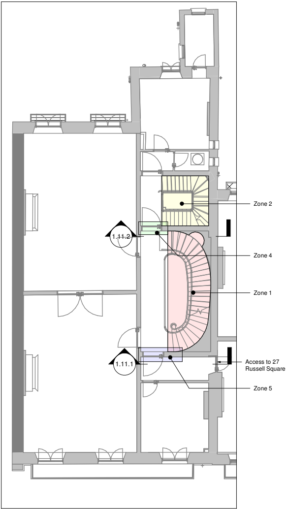
1 First Floor Plan 1 : 100
