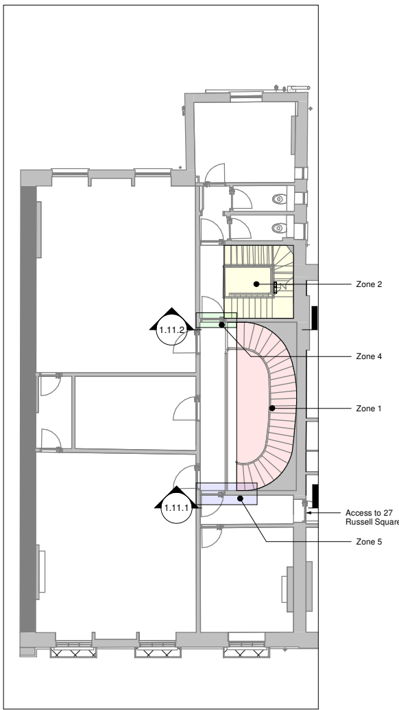
2 Second Floor Plan 1 : 100
