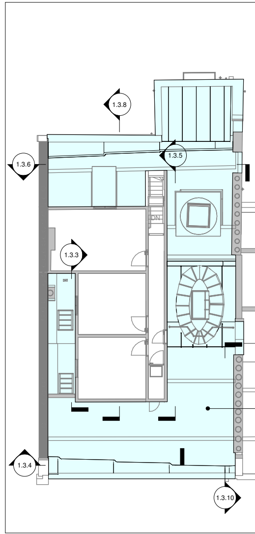
1 Roof Plan- 42.06 1 : 100
