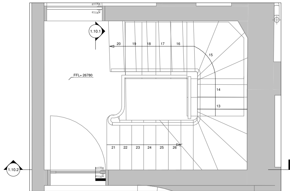
1 Ground Floor Small Staircase Plan 1 : 20
