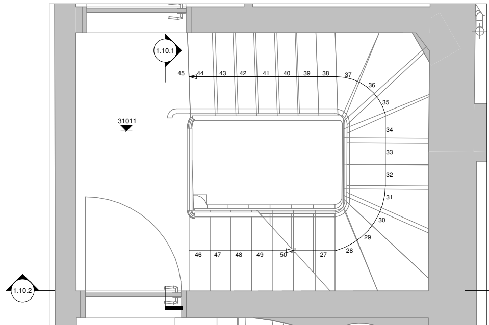
2 First Floor Small Staircase Plan 1 : 20
