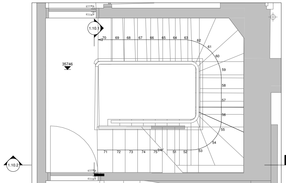
3 Second Floor Small Staircase Plan 1 : 20
