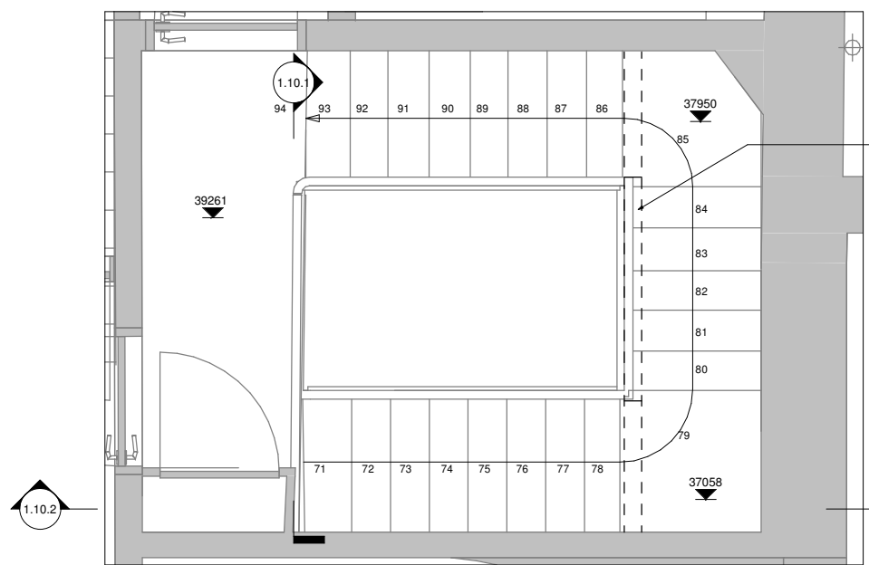
4 Third Floor Small Staircase Plan 1 : 20
