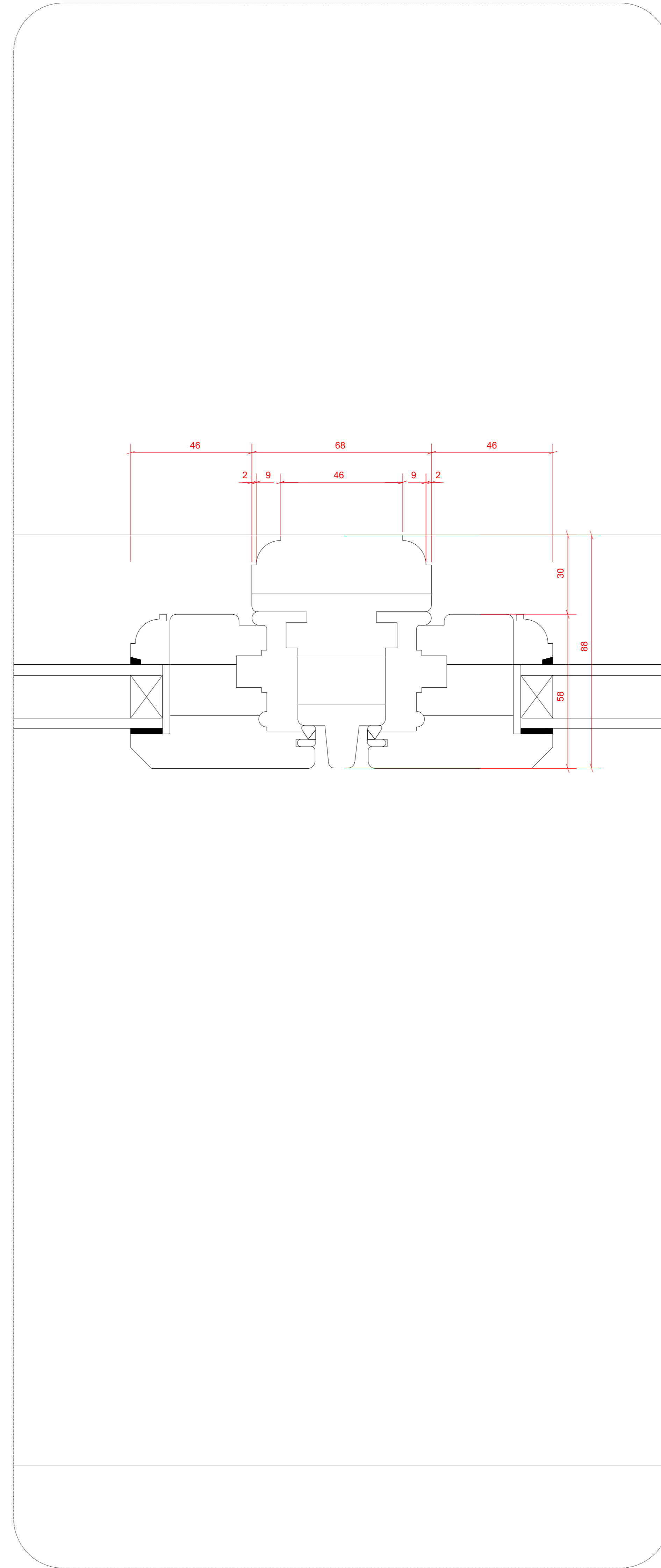
400_305 or Typical Casement Window Glazing Bar Detail Scale 1:1
