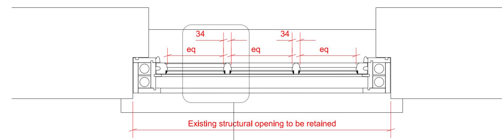
400_305.02 WINDOW TYPE G RW.07, RW.08, RW.17, scale 1:10 New sash windows without shutters
