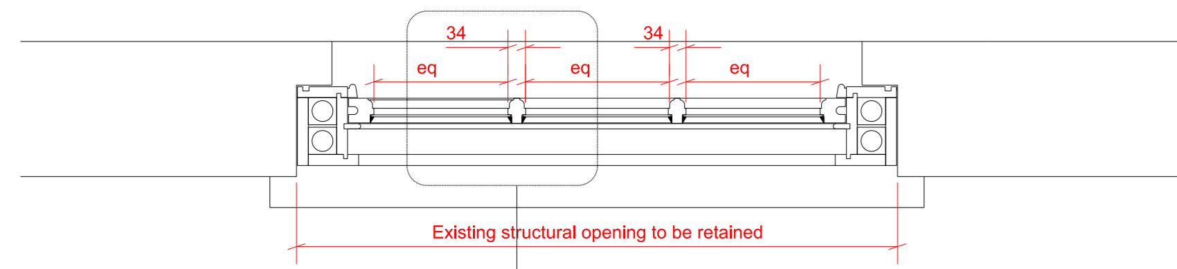
400_305.01 WINDOW TYPE F RW.01, RW.02, RW.03, RW.04, RW.05, RW.06, scale 1:10 New sash windows without shutters
