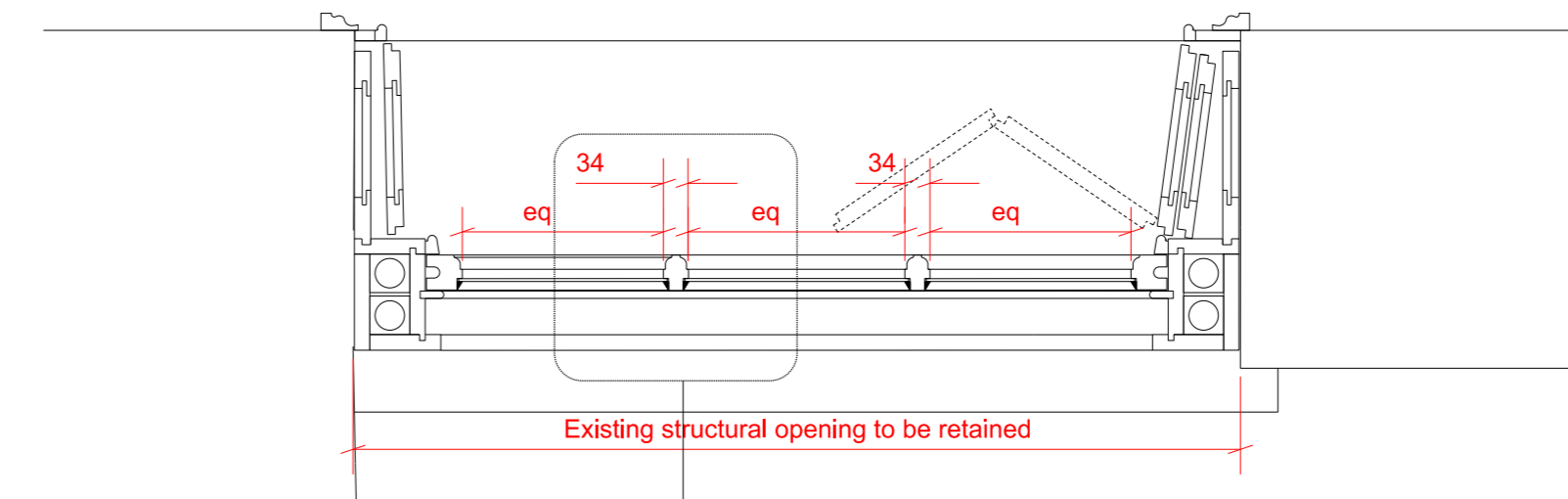
400_305.03 WINDOW TYPE H RW.12, scale 1:10 New sash window with shutters
