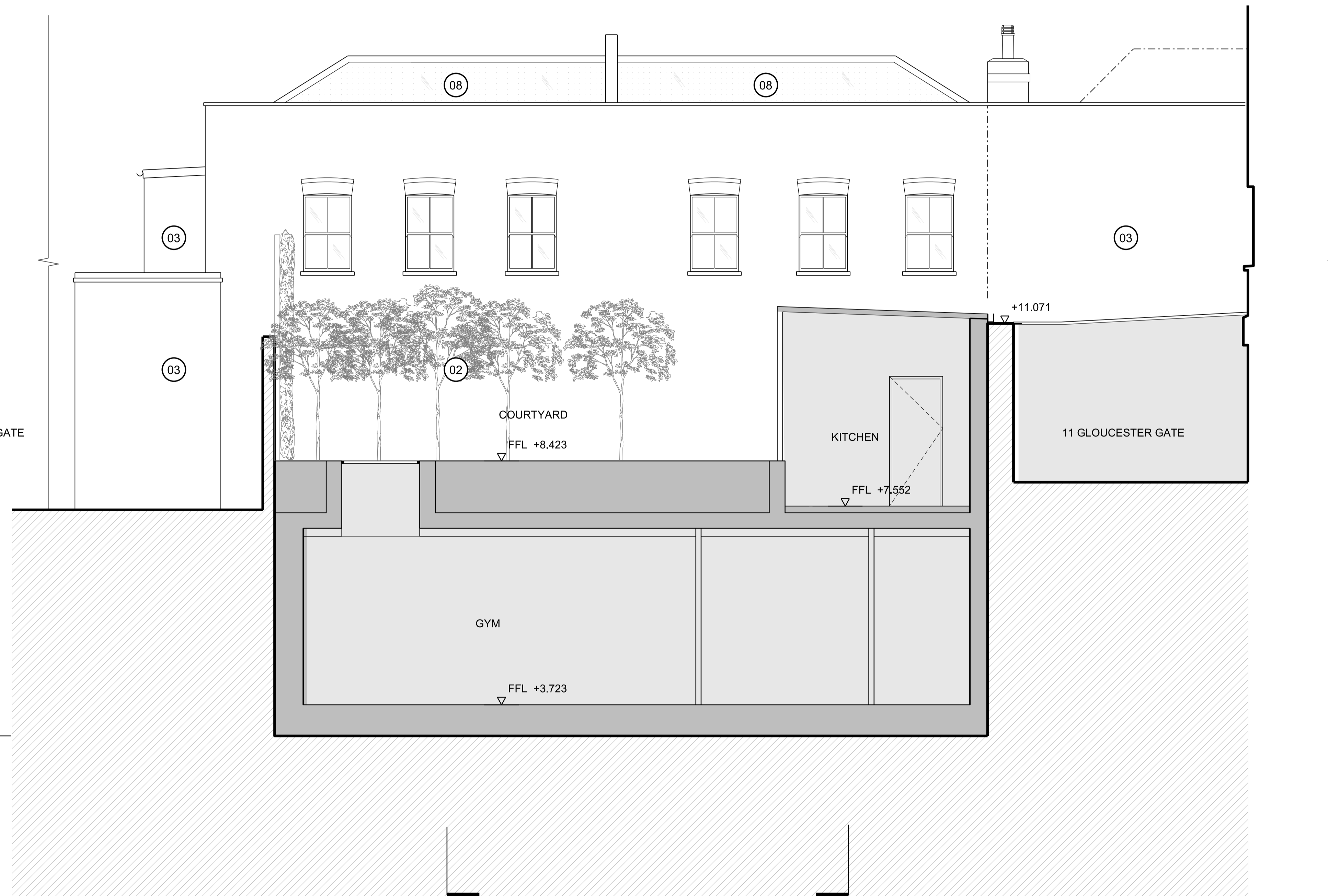
01 Proposed section D 1:50
