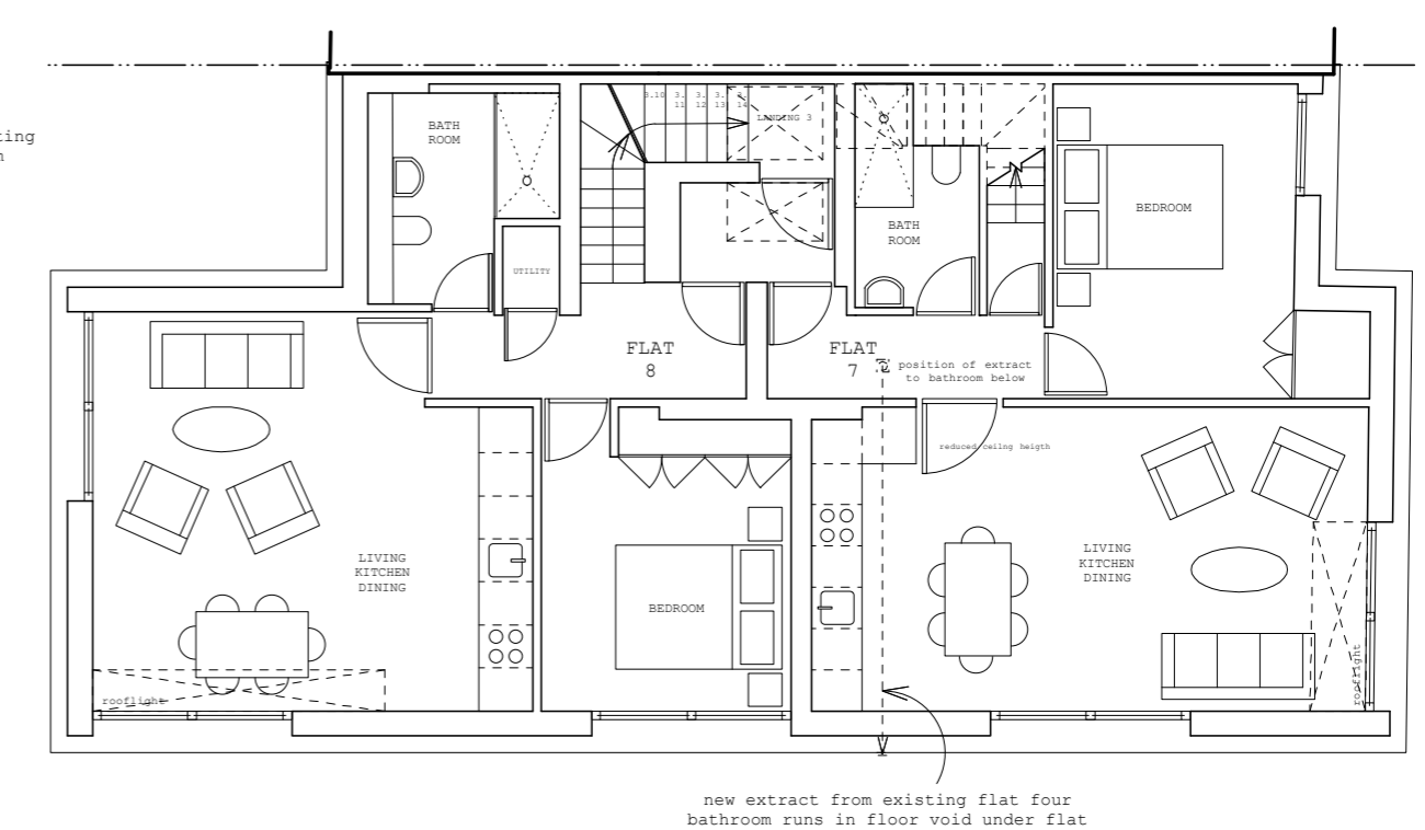
04 4F Plan
