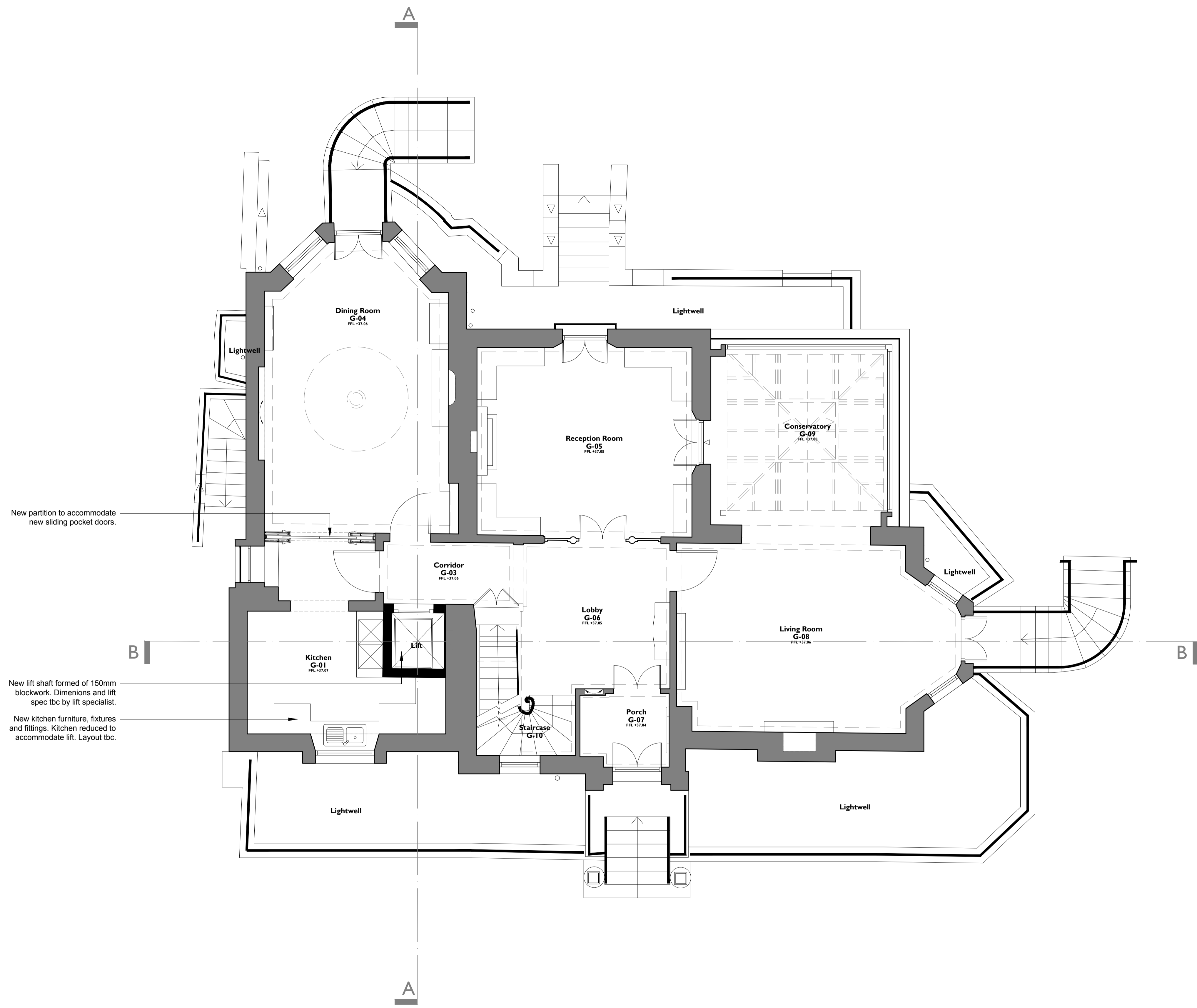
I 202 As Proposed: Ground Floor Plan 1:50@A1, 1:100@A3
