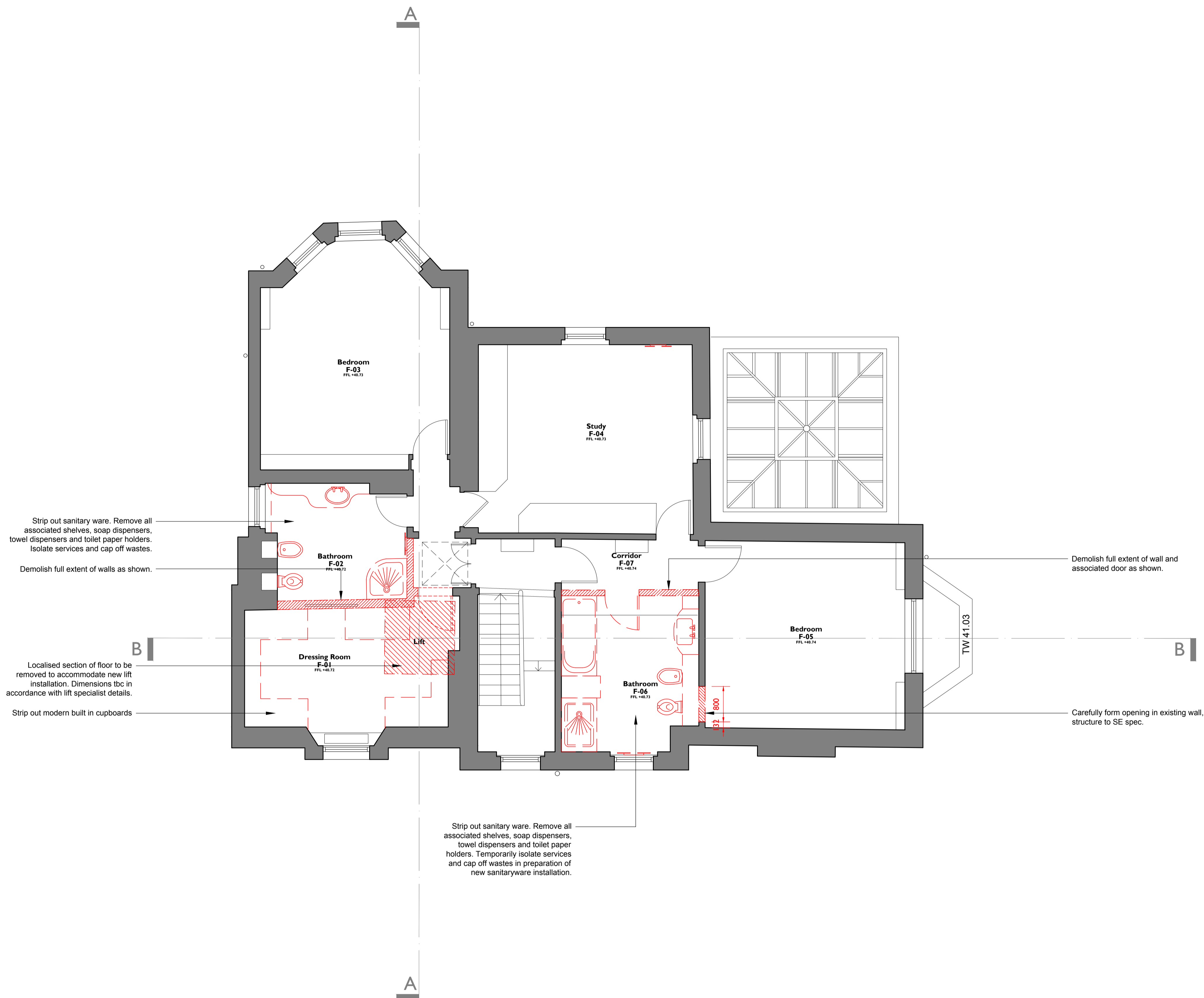
I Demolition: First Floor Plan 133 1:50@A1, 1:100@A3
