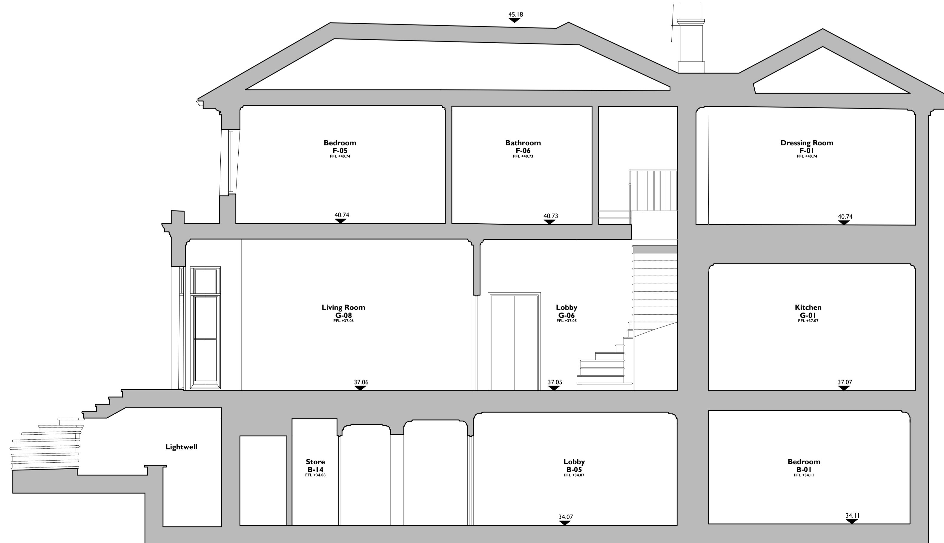
2 As Existing: Section BB 105 1:50@A1, 1:100@A3
