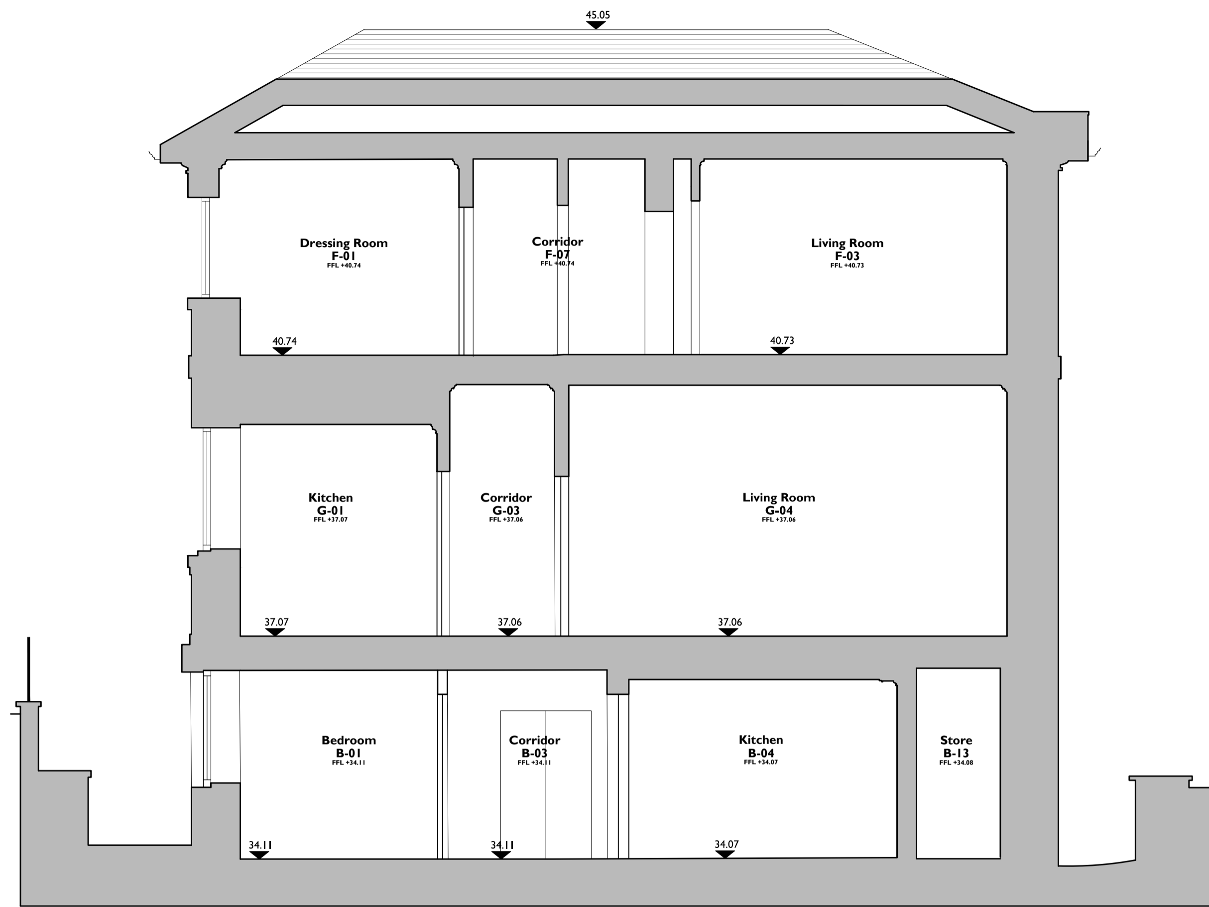
1 As Existing: Section AA 105 1:50@A1, 1:100@A3
