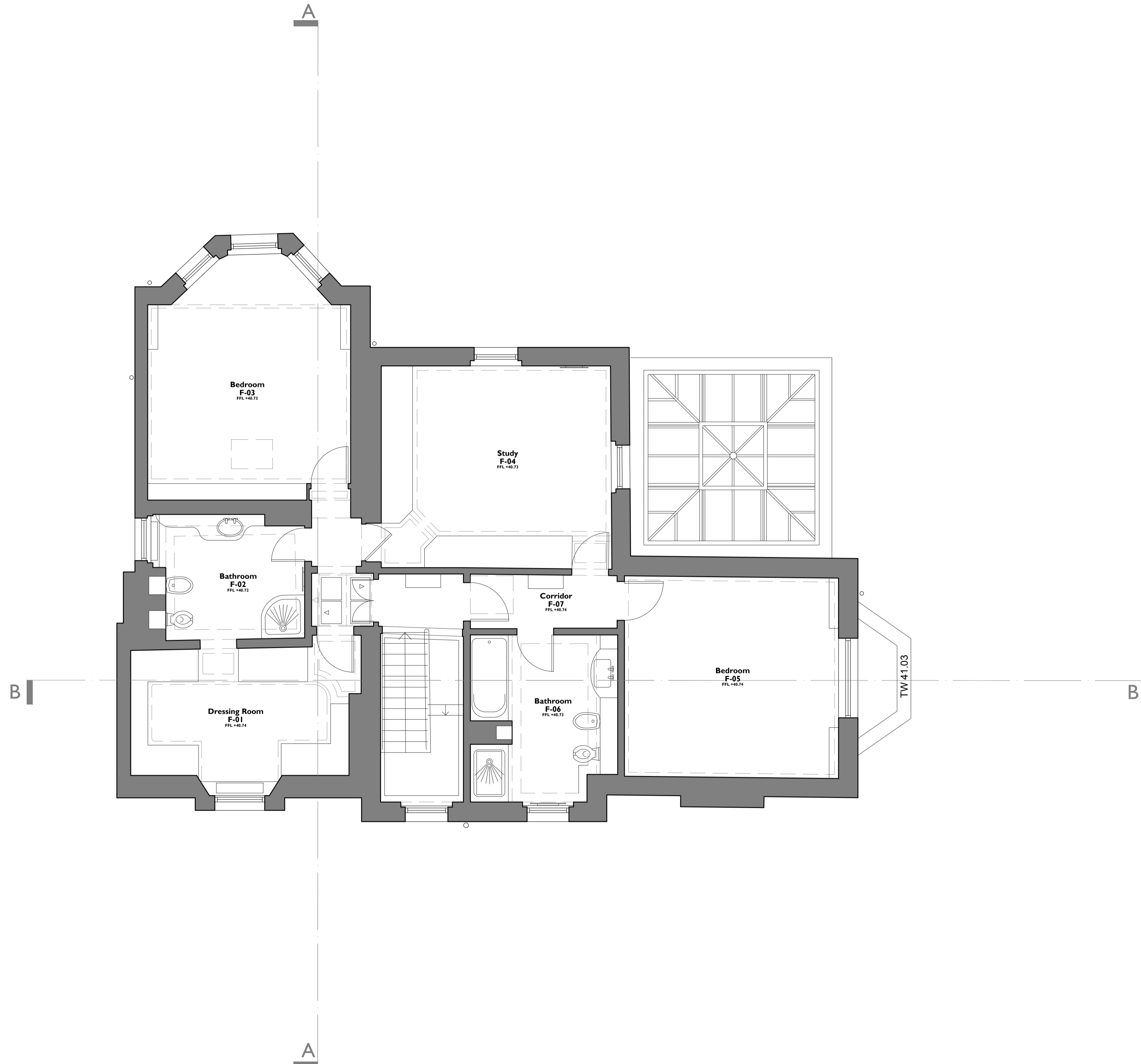
I 103 As Existing: First Floor Plan 1:50@A1, 1:100@A3
