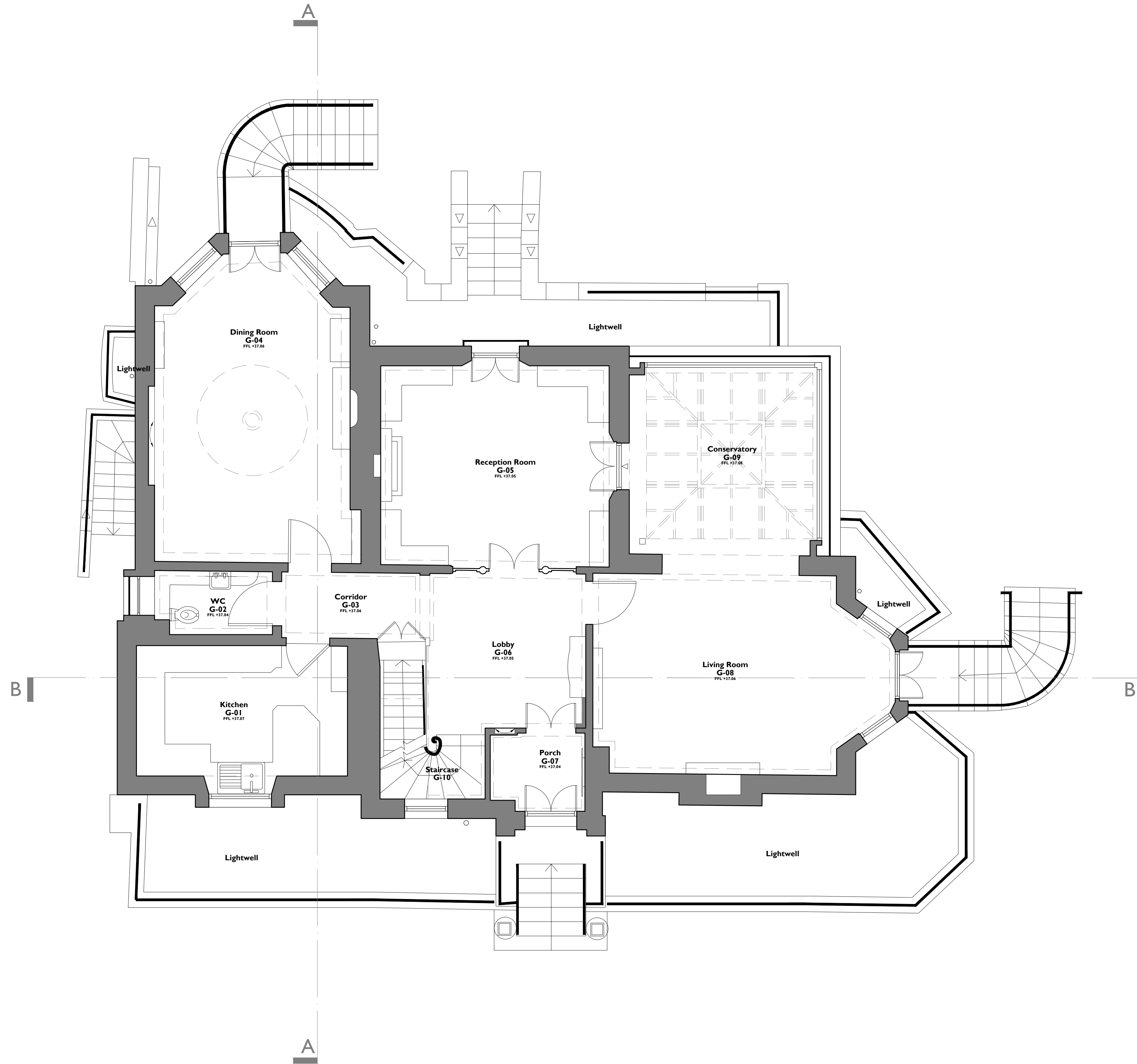
I 102 As Existing: Ground Floor Plan 1:50@A1, 1:100@A3
