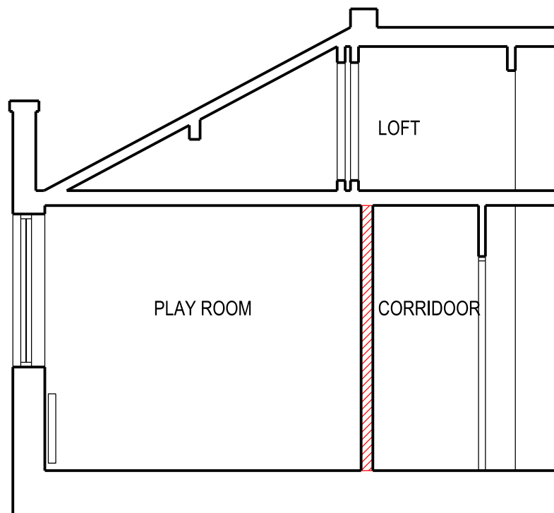
1 1:50 EXISTING SECTION A
