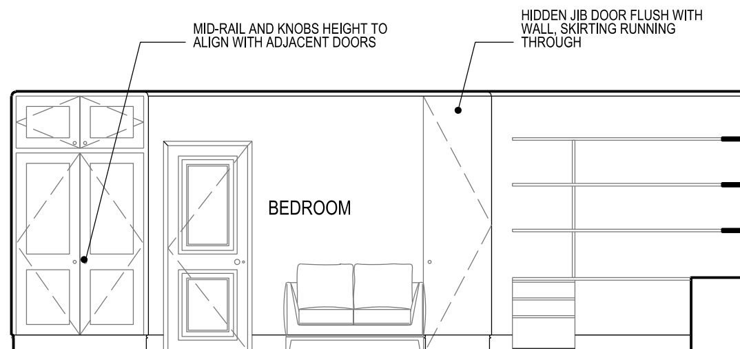
4 1:50 PROPOSED SECTION D
