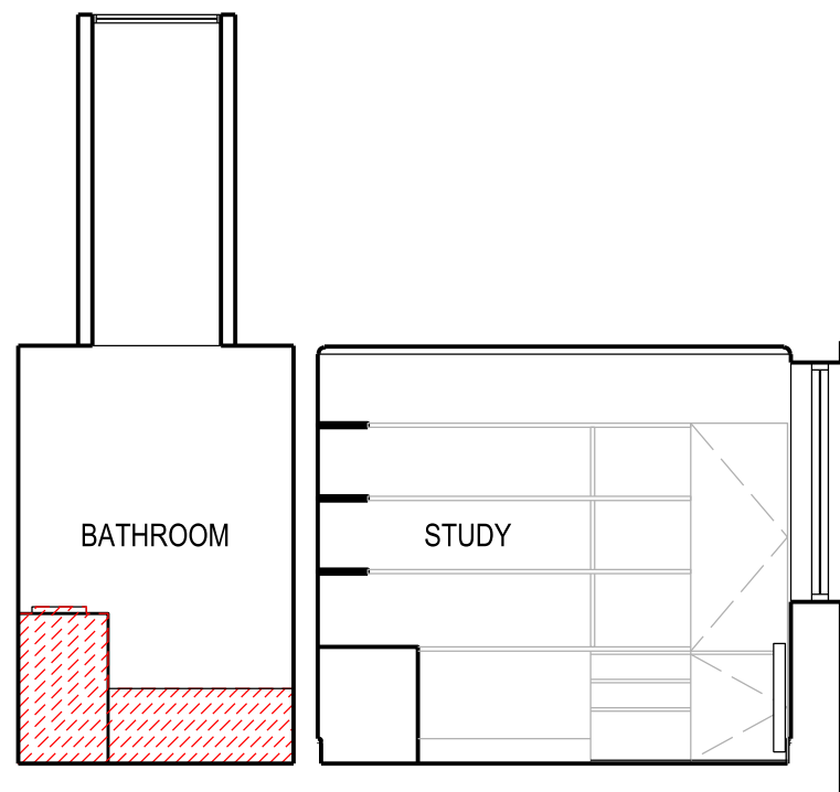
2 1:50 EXISTING SECTION B
