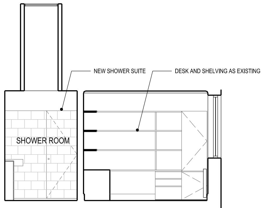
2 1:50 PROPOSED SECTION B
