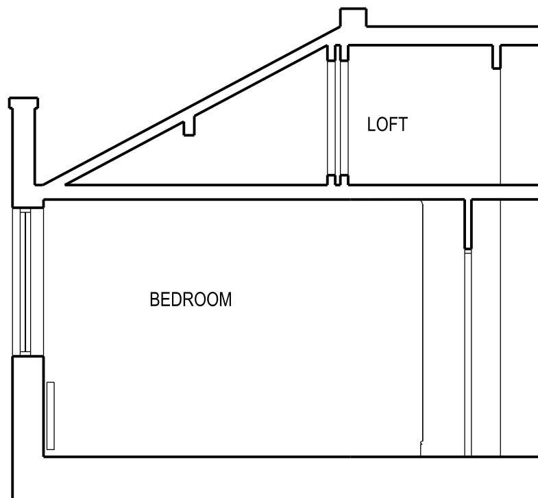
1 1:50 PROPOSED SECTION A
