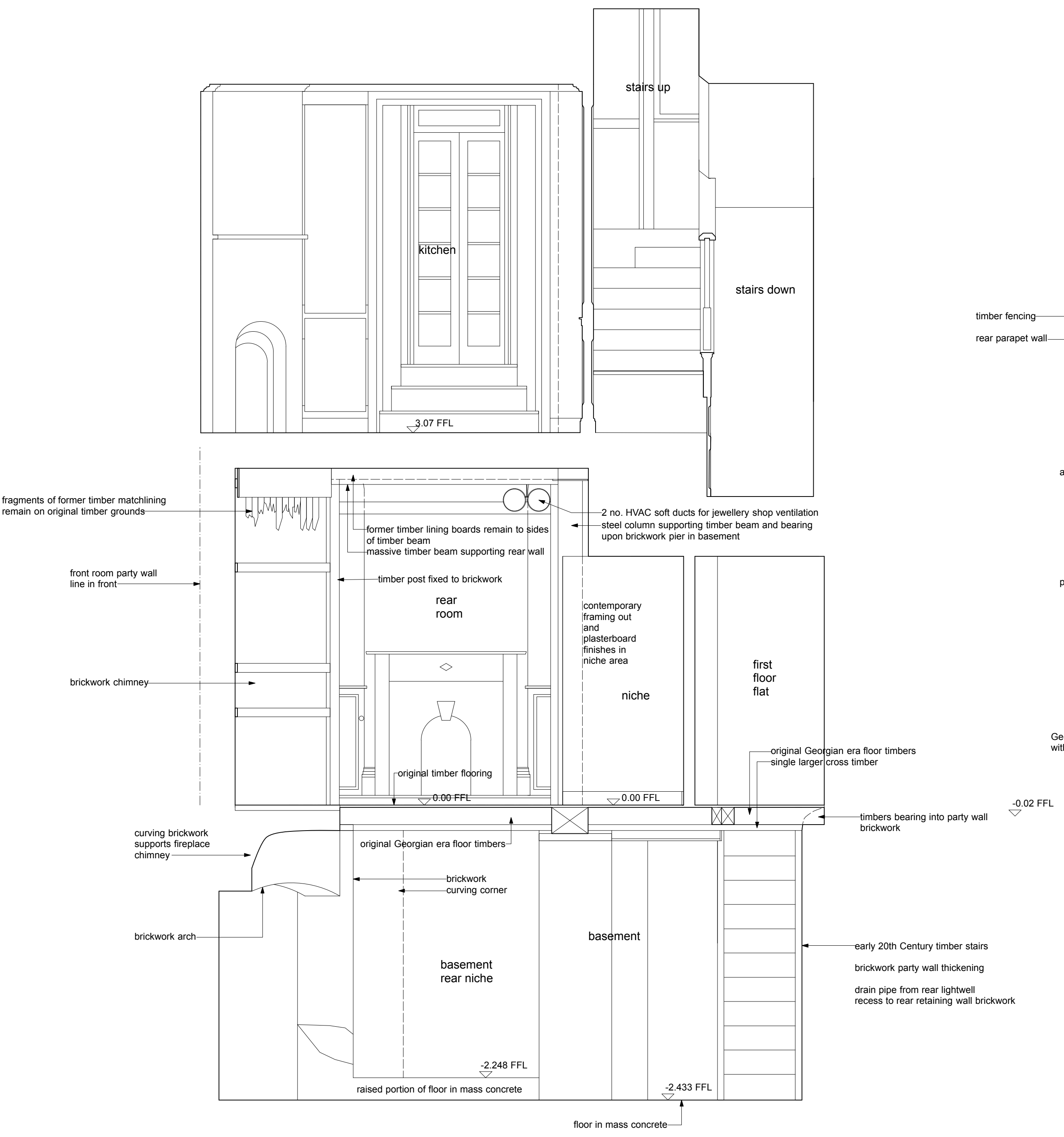
detailed existing section F-F 1:25
