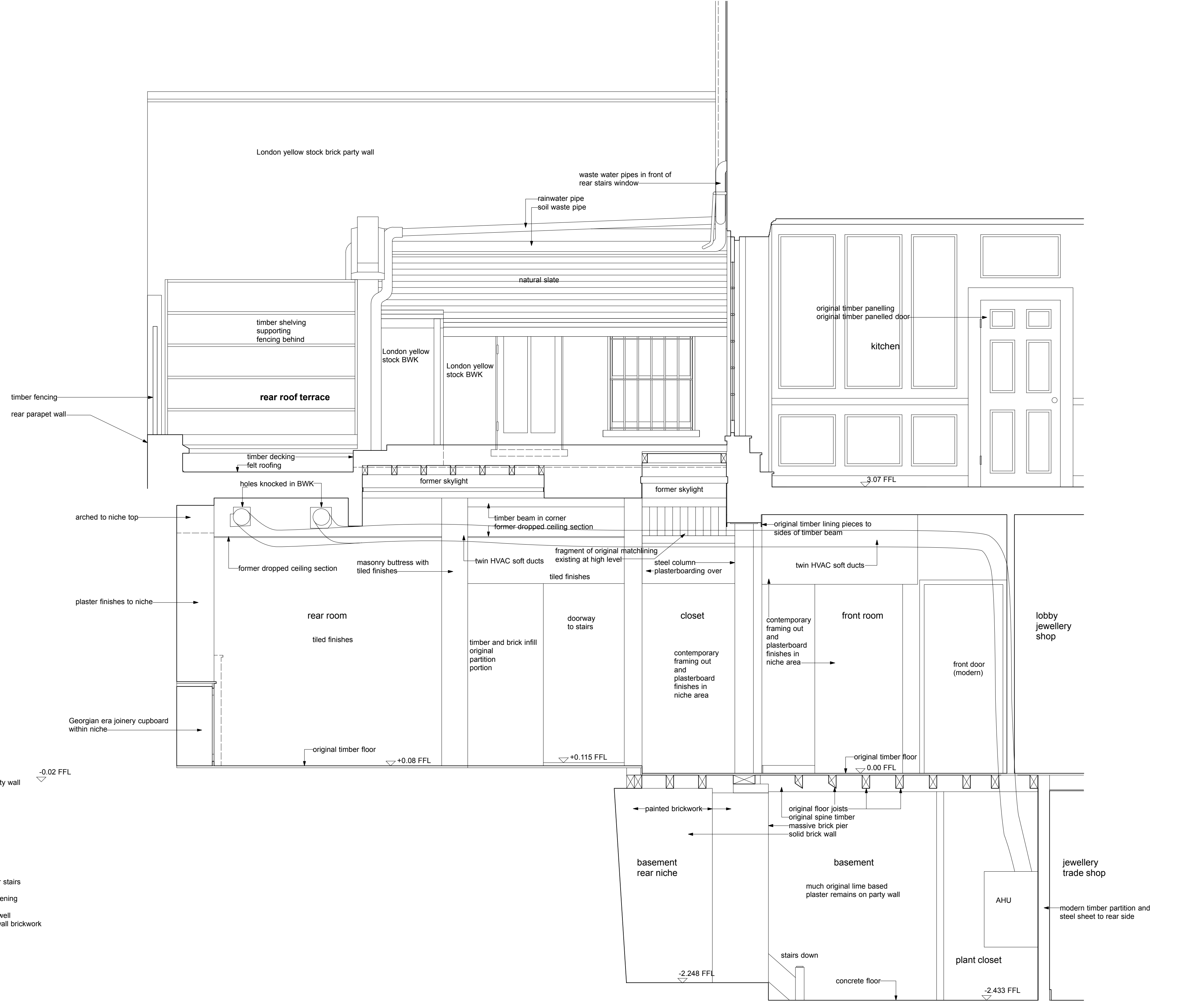
detailed existing section i-i 1:25
